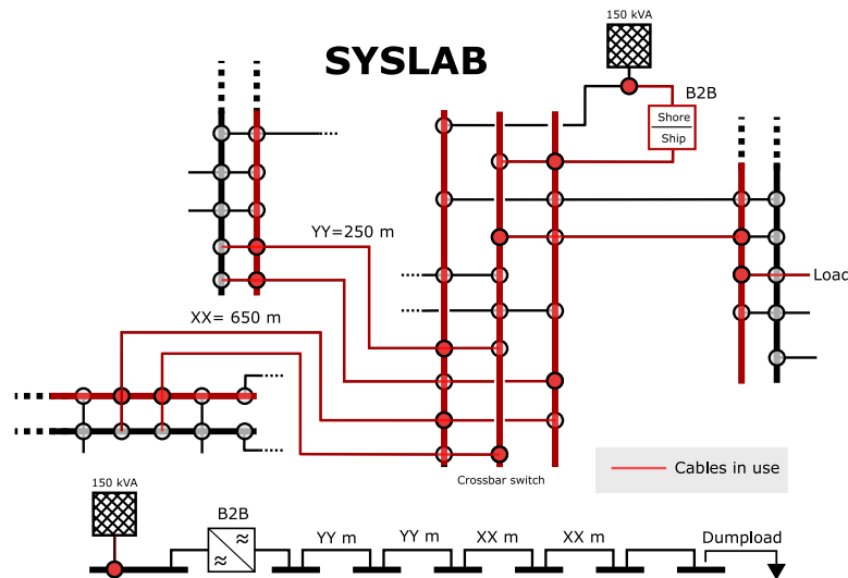
Figure 4. SYSLAB topology.
