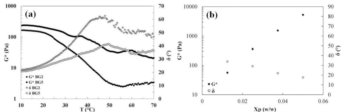
Fig. 8. (a) Complex modulus ( G^* ) and phase angle ( \delta ) at 1 Hz as a function of temperature obtained at a heating rate of 1 °C/min for pectin/policosanol/olive oil based bigels with 5 wt% organogelators (BG2) and 10 wt% organogelators (BG5), reprinted with permission from ref. (F. R. Lupi et al., 2016), Copyright [2016], Elsevier, (b) complex modulus ( G^* ) and phase angle ( \delta ) at 1 Hz and 25 °C as a function of hydrogelator (pectin) concentration for pectin/policosanol/olive oil based bigels, reprinted with permission from ref. (Francesca R Lupi, De Santo, et al., 2017), Copyright [2017], Springer Nature.
