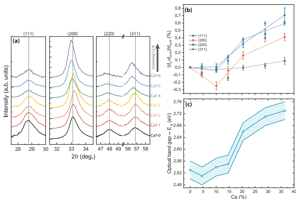
Figure 3. (a) GI-XRD patterns for (\text{Ca}_x\text{Y}_{1-x})\text{H}_x\text{O}_y with different Ca content. Vertical gray lines are references for the reflections of the 0% Ca sample. (b) Relative change in d -spacing for different reflections as a function of Ca content showing the increase in strain for Ca contents > 15%, and that the strain is not isotropic. Lines are guides for the eye. (c) Change in the optical band gap energy as a function of Ca content, showing an increase above 15% Ca.
