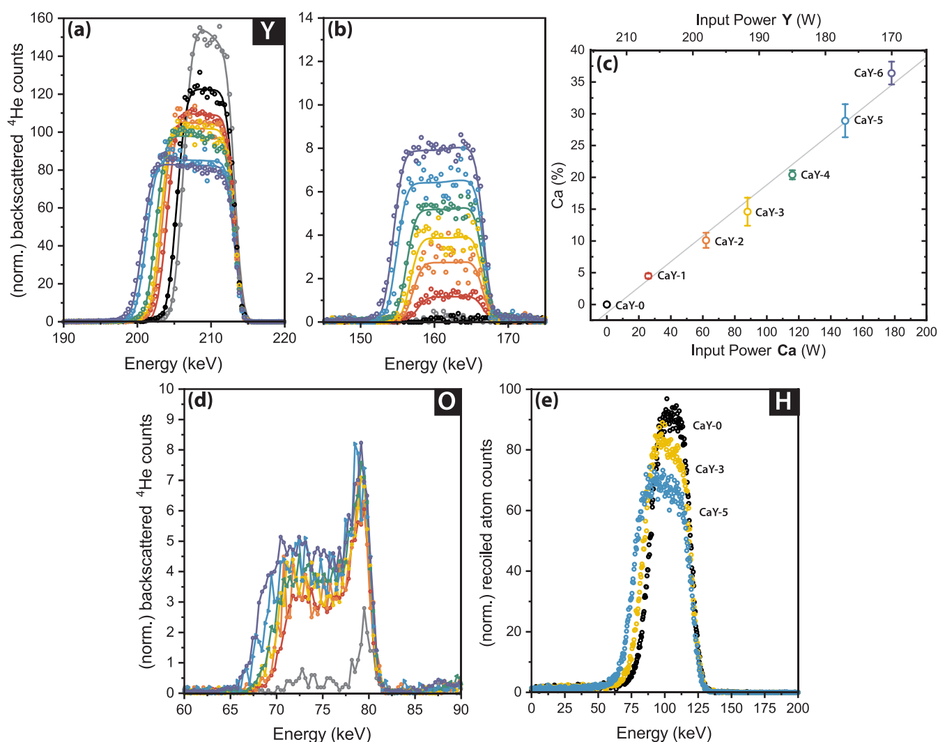
Figure 2. Overview of the compositions of Ca-doped oxyhydride thin films ( \text{Ca}_x\text{Y}_{1-x}\text{H}_x\text{O}_y ). For (a) and (b), the lines are from simulations of the composition using SIMNRA. RBS data for (a) yttrium, (b) calcium, and (d) oxygen are shown for \text{YH}_{1.9+\delta} and a series of oxyhydrides with gradually higher Ca content, where the black points are for CaY-0 (0% Ca) and purple points are for CaY-6 with the most Ca. (c) Ca content calculated from RBS along with the input power to the Ca and Y targets during cosputtering showing the linear relationship. (e) ERD results for hydrogen as more calcium is added to yttrium oxyhydride. All RBS and ERD data are normalized to account for differences in accumulated charge.
