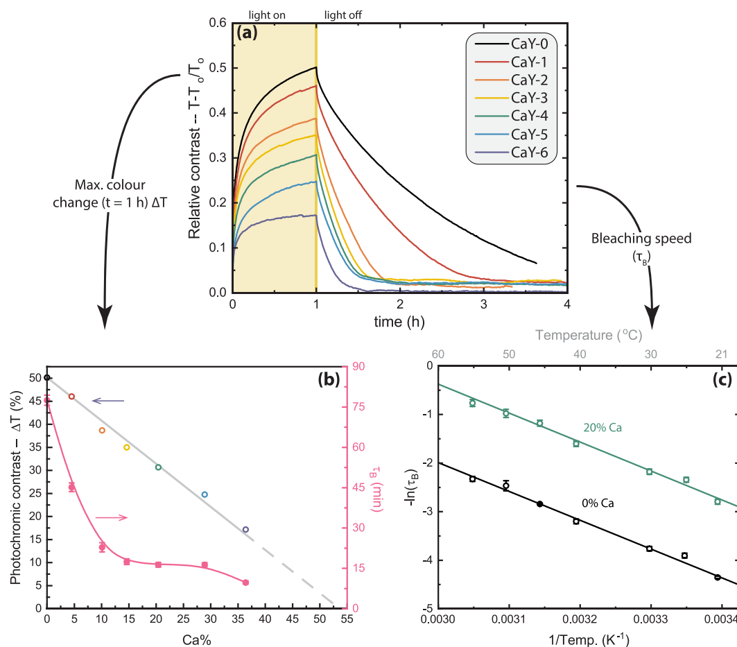
Figure 4. (a) Relative contrast for (\text{Ca}_x\text{Y}_{1-x})\text{H}_x\text{O}_y thin films with varying Ca content. When the sample is transparent, the relative contrast is 0. During 1 h of illumination, the contrast increases and later decreases back to 0 when the illumination is stopped. (b) (left y-axis) The maximum relative contrast as a function of Ca content. Extrapolation of the linear relationship leads to a prediction of 0% contrast when the Ca doping concentration is \sim 54\% . (right y-axis) The bleaching speed ( \tau_B ) becomes faster with the addition of Ca, although following a nonlinear relationship. (c) Arrhenius plot of the bleaching speed for (\text{Ca}_x\text{Y}_{1-x})\text{H}_x\text{O}_y thin films containing 0 and 20% Ca, showing that differences in bleaching speed are not due to an altered activation energy of the process but are dependent on the pre-exponential factor.
