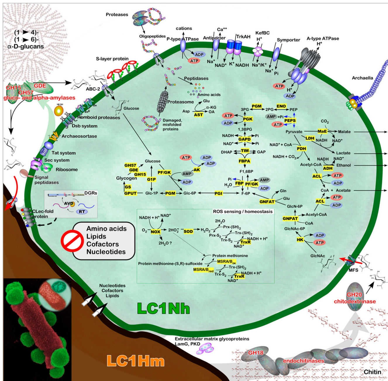
Fig. 5. Reconstruction of central metabolic and homeostatic functions of Ca. Nanohalobium constans LC1Nh based on genomic, proteomic, targeted metabolomic, and physiological analyses. Enzymes involved in energy production and in reactive oxygen species (ROS) homeostasis/redox regulation are highlighted in yellow. Chitin degradation enabled by seven extracellularly expressed GH18 endochitinases and one GH20 chitodextrinase of the host, is indicated by the gray arrow in the lower-right part of the figure. Depolymerization of (1 → 4)- and (1 → 6)-α-D-glucans by two experimentally confirmed extracellularly expressed glucoamylases of Ca. Nanohalobium constans LC1Nh is shown with the green arrow in the upper-left part of the figure. The mutualistic uptake of the formed sugars is indicated by the red arrow. Compounds abbreviations: Asp, aspartate; α-KG, α-ketoglutarate; 1,3BPG, 1,3-bisphosphoglycerate; CoA, coenzyme A; DHAP, dihydroxyacetone phosphate; F-6P, fructose-6-phosphate; F1,6BP, fructose-1,6-bisphosphate; Glc-6P, glucose-6-phosphate; Glc-1P, glucose-1-phosphate; GlcNAc, N-acetyl-glucosamine; GlcNAc-6P, N-acetyl-glucosamine-6-phosphate; GlcN-6P, N-glucosamine-6-phosphate; Glu, glutamate; Gln, glutamine; GAP, glyceraldehyde-3-phosphate; OA, oxaloacetate; 3PG, 3-phosphoglycerate; 2PG, 2-phosphoglycerate; PEP, phosphoenolpyruvate; Prx, peroxiredoxin; Trx, thioredoxin. Genes and systems abbreviations: ACL, acetate-CoA ligase; ADH, alcohol dehydrogenase; AK, adenylate kinase; AST, aspartate aminotransferase; AVD, diversity-generating retroelement protein; Clec, C-type lectin fold; DGR, diversity-generating retroelements system; Dsb, disulfide bond formation; GNFAT, glucosamine-fructose-6-phosphate aminotransferase; ENO, enolase; FBPA, fructose-1,6-bisphosphatase; G1P, glucose-1-phosphatase; GAPD, glyceraldehyde-3-phosphate dehydrogenase; GDE, glycogen debranching enzyme; GH, glycogen hydrolase; GNPAT, bifunctional UDP-N-acetylglucosamine pyrophosphatase; GPAT, UTP-glucose-1-phosphateuridylyltransferase; GS, glycogen synthase; HK, gluco(hexo)kinase; LamG, laminin G domain; LDH, lactate dehydrogenase; A, malic enzyme; MFS, major facilitator superfamily; MSRA, peptide-methionine (S)-S-oxide reductase; MSRB, peptide-methionine (R)-S-oxide reductase; NOX, pyridine nucleotide-disulphide oxidoreductase; PDH, pyruvate dehydrogenase; PEPs, phosphoenolpyruvate synthase; PGI, glucose-6-phosphate isomerase; PGM, 2,3-bisphosphoglycerate-independent phosphoglycerate mutase; PGK, phosphoglycerate kinase; PF/GK, phosphofructokinase/glucokinase; PKD, polycystic kidney disease; ROS, reactive oxygen species; RT, reverse transcriptase; SOD, superoxide dismutase; TIM, triosephosphate isomerase; TrxR, thioredoxin reductase. Details on genes and systems abbreviations are provided in SI Appendix, Table S7 .
