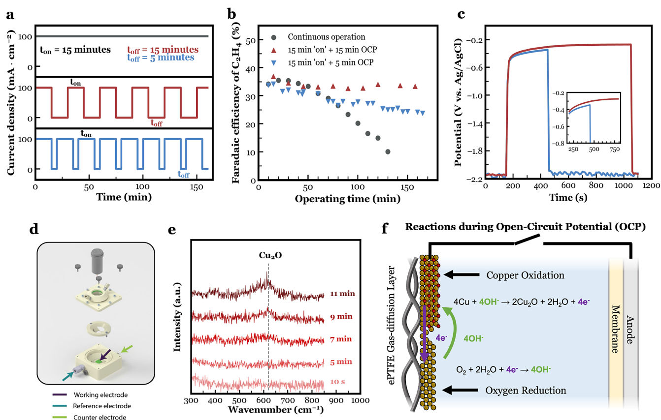
Figure 2. (a) The different performed chronopotentiometry experiments. A constant current density at -100 \text{ mA} \cdot \text{cm}^{-2} (black). A pulsed current with 15 min at -100 \text{ mA} \cdot \text{cm}^{-2} , followed by 15 min at OCP (red). A pulsed current with 15 min at -100 \text{ mA} \cdot \text{cm}^{-2} , followed by 5 min at OCP (blue). (b) FE of \text{C}_2\text{H}_4 as a function of time for the current profiles depicted in (a). (c) Change in OCP value with time during the oxidative pulse. (d) The in situ Raman spectroscopy setup. (e) Raman spectroscopy data showing the intensity of the \text{Cu}_2\text{O} signal at different OCP times. (f) The half reactions associated with the formation of \text{Cu}_2\text{O} during OCP.
