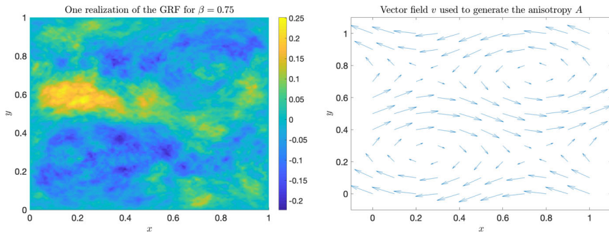
Fig. 3 Left : One realization of the generalized Whittle–Matérn field \mathcal{Z}^\beta on \mathcal{D} = (0, 1)^2 as considered in Sect. 9.2. Right : The vector field v: \mathcal{D} \rightarrow \mathbb{R}^2 employed in A(x, y) = c \text{Id}_{\mathbb{R}^2} + v(x, y)v(x, y)^\top \in \mathbb{R}^{2 \times 2} , for x, y \in [0, 1] , to generate the anisotropic coefficient A of the differential operator L in (12)
