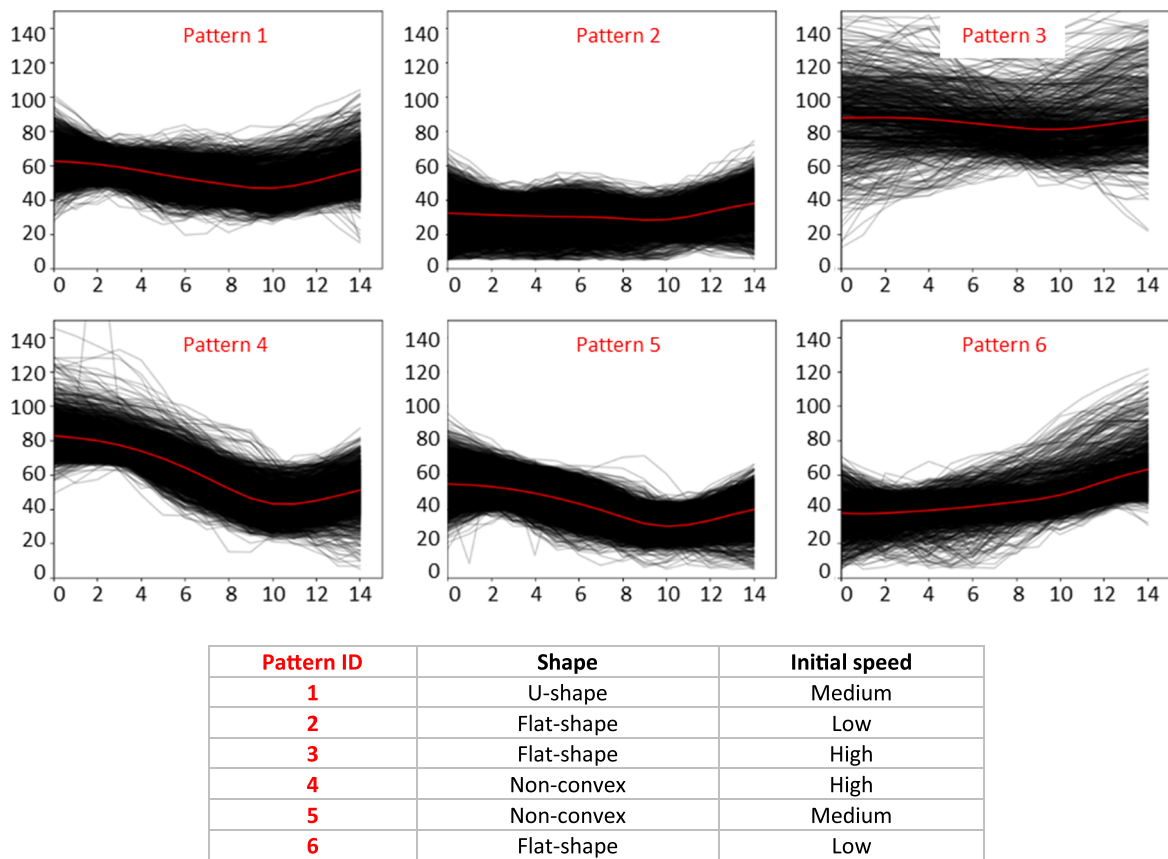
Fig. 4. Results of the 6 different speed patterns identified during harsh cornering events (Y axis: Speed, X axis: time, harsh event occurs at the 11th second of the X-series).
