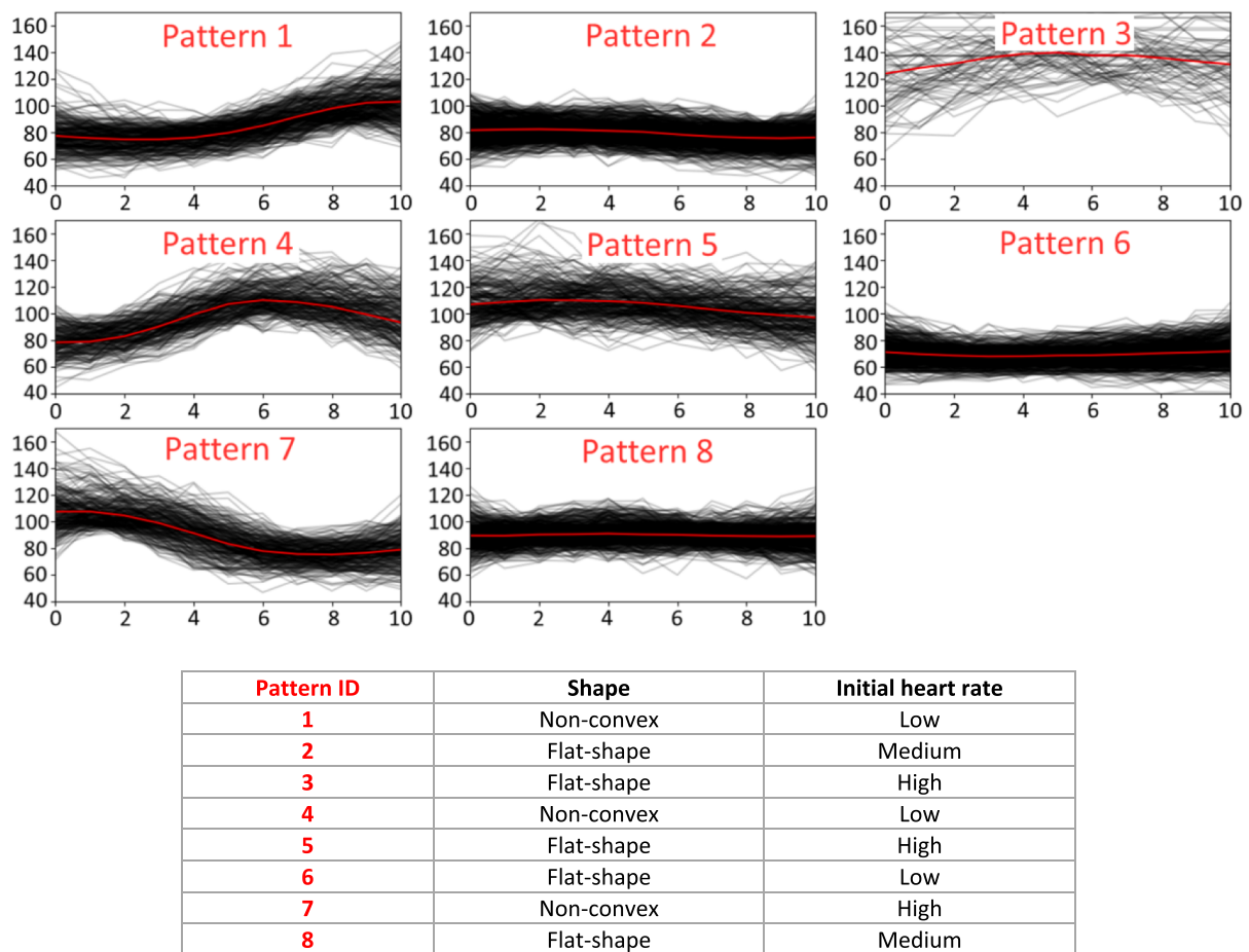
Fig. 7. Results of the 8 smoothed heart beat patterns identified during harsh cornering events, using 30 heart beats/minute difference threshold (Y axis: Heart rate/ minute, X axis: time, harsh event occurrence is included in all seconds between 7th to 10th of the X-series).
