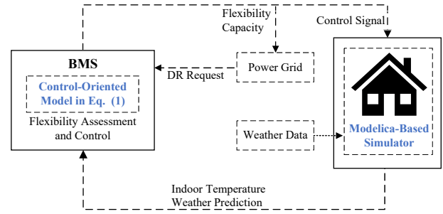
Fig. 2. Simulation Diagram.
