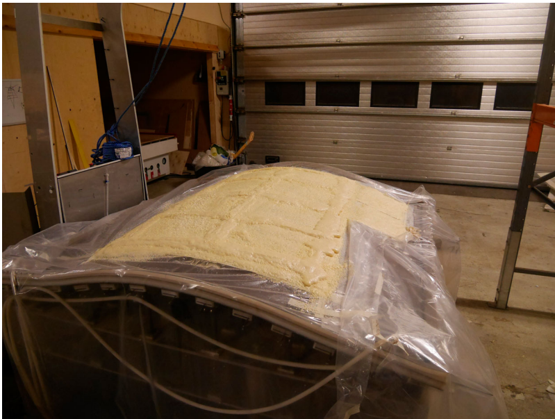
Figure 16. Curing of the HDPU foam on the flexible table.
