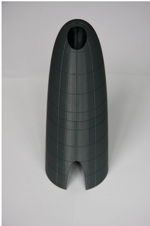
Figure 34. 3D printed thermoplastic model of the selected 1:500 scale hyperbolic shell, without entrance.
