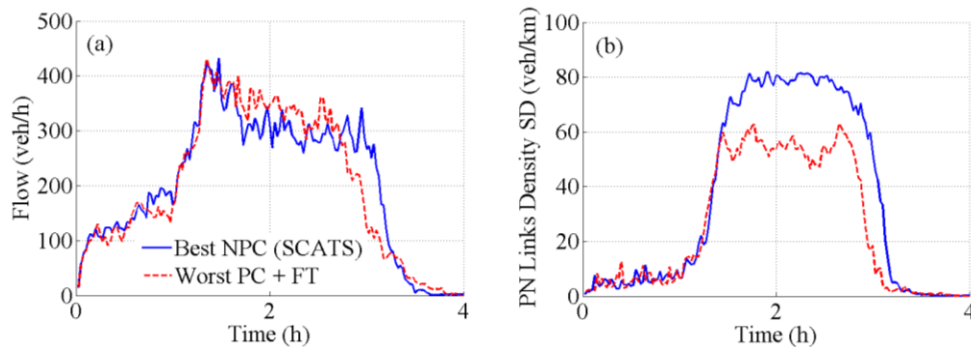
Figure 11 (a) PN average flow vs. time for the best NPC (SCATS) and the worst PC + FT performance among 10 runs; (b) PN link density SD vs. time for the best NPC (SCATS) and the worst PC + FT performance among 10 runs
