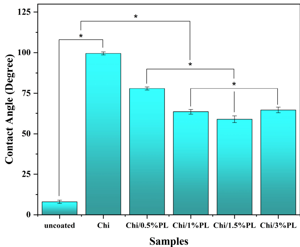
Figure 7. The result of contact angle measurements for anodized \text{Ti}_6\text{Al}_4\text{V} surface and surfaces, coated with chitosan- x\% \epsilon -PL ( 0.5 < x < 3.0\% ) layer. (*: p < 0.05 , The data underwent analysis through a one-way ANOVA method, followed by Tukey's post-hoc test for further evaluation. Statistical significance was established at a threshold of p < 0.05 to identify any meaningful differences).
