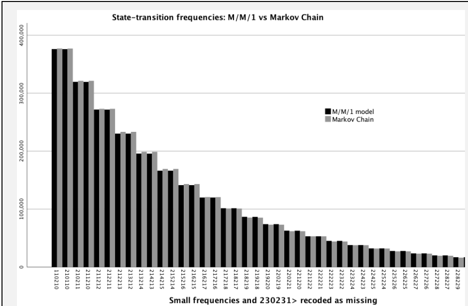
Figure 3.8. The frequency distributions of the recoded state transitions of M/M/1 model and Markov Chain for 100 repetitions with 50,000 state-trace length
