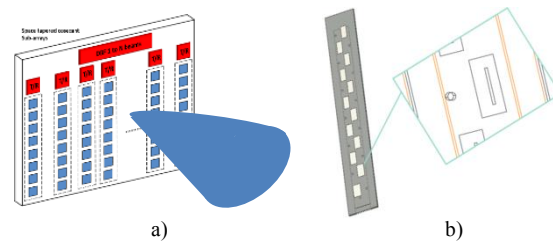
Fig. 2. Array of vertical shaped beam sub-arrays
