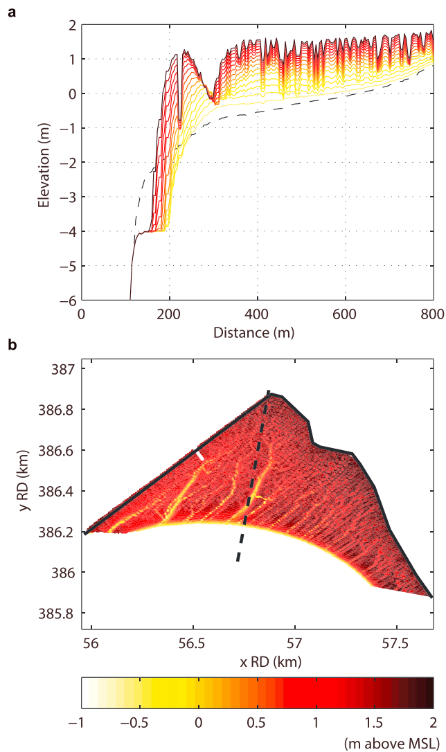
Figure 14. (a) The modeled evolution of the indicated transect in panel b, without wind waves ( \tau_{cr}=0.2 & C_0 = 5 mg/L). The cross-section of the initial bathymetry (2015 data) is indicated by the dashed black line and the evolution occurs from yellow toward dark red, with time intervals of 25 years and a total time span of 375 years. (b) Map of the bathymetry after 375 years of morphodynamic evolution. A morphological factor of 1,000 is applied.
