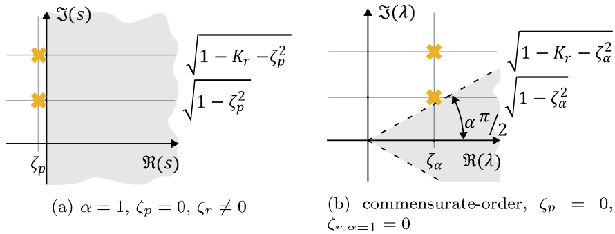
Fig. 3 Locations of approximated (pseudo)poles of a single unit cell for a) \omega \gg \omega_r and b) \omega \approx \omega_r or \omega < \omega_r . The absolute values of poles are scaled to enable comparison
