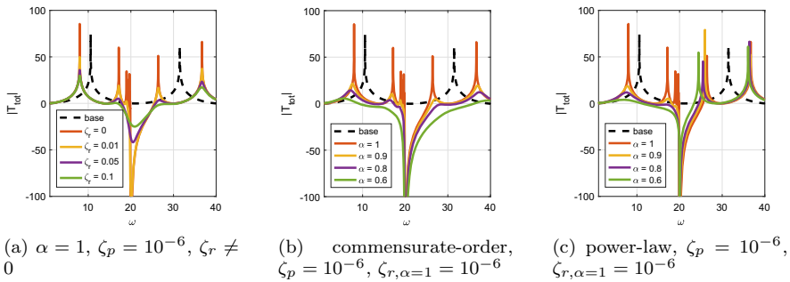
Fig. 6 Transmissibility of a finite metastructure of 10 cells with (a) integer-order and (b) commensurate-order or (c) power-law fractional-order resonators. The base chain of the metastructure is nearly undamped
