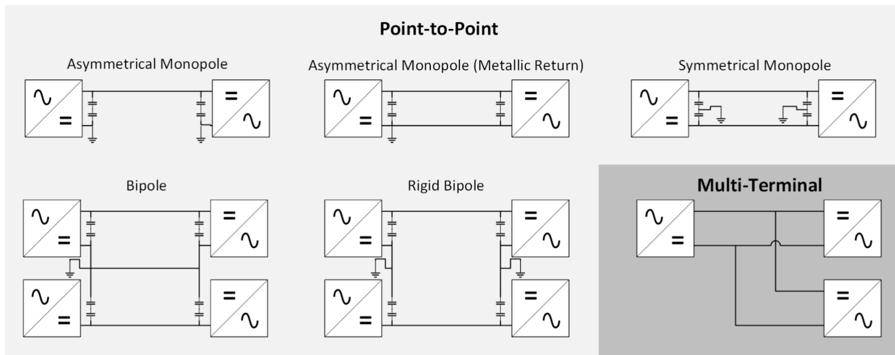
FIGURE 4. HVDC topologies.
