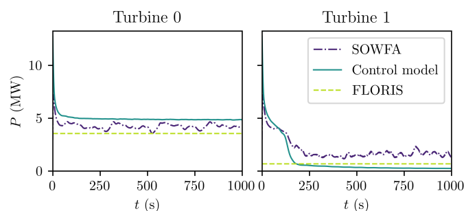
Figure 4: Power development over time.
