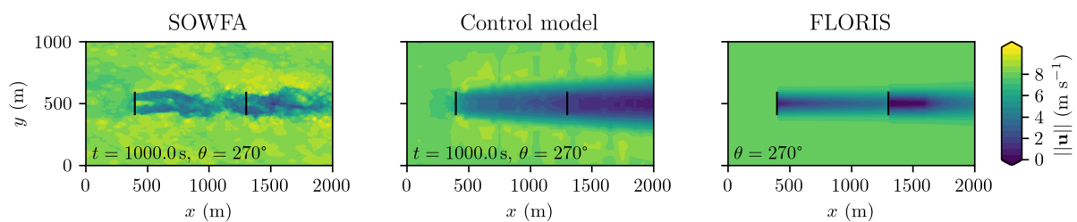
Figure 3: Two-turbine array with steady 8.0 \text{ ms}^{-1} inflow from left side, as illustrated in Figure 2a. Comparing results from SOWFA with a turbulent inflow on the left, steady-state results from FLORIS on the right, and planar flow results from the new control model in the centre.
