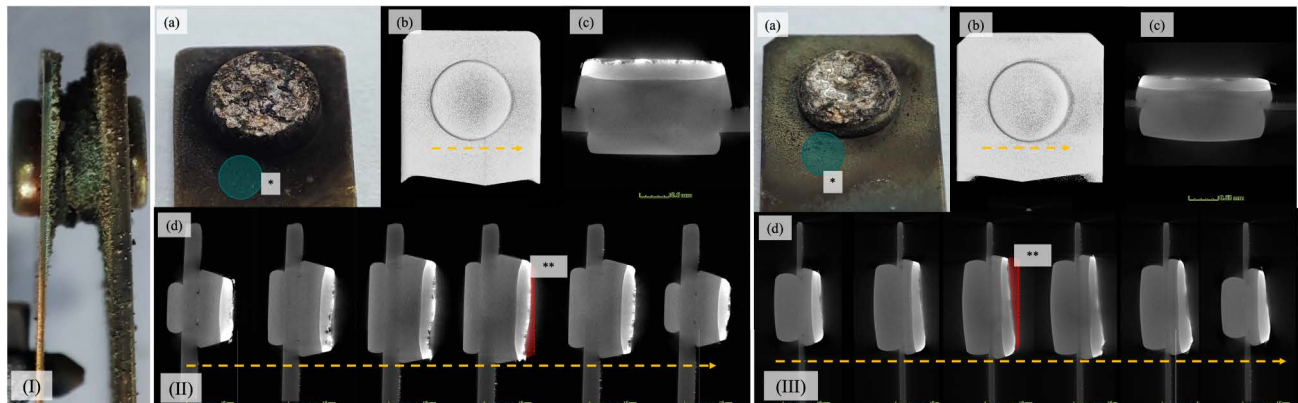
FIGURE 12. (I) Example of stuck-closed EMR contacts (unsealed), due to contact welding; (II) (a) photography of the static contact carrier (anode) after failure; (b), (c) and (d) CT-Scans and cross-sections (the brighter coloured grey area on the contact rivet is oxidised silver and the silver contact plating material, while the darker grey area is the copper contact rivet body); (*) sputtered, eroded contact material; (**) dashed red line represents the contact height of the new EMR contact; (III) photography and CT-Scan of the moving contact carrier (cathode) after failure, cf. (II).
