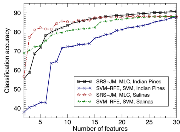
Fig. 11 The classification accuracy obtained by a filter approach, i.e., features identified by SRS-JM and the classification with MLC and one wrapper approach (SVM-RFE) for two datasets. The legend gives in each row the feature identification algorithm, the classification method, and the dataset used, respectively.
