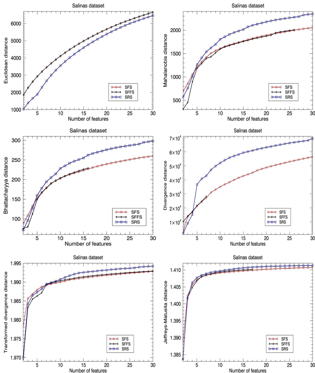
Fig. 8 The mean separability distance of the features obtained with different algorithms for the Salinas dataset.
