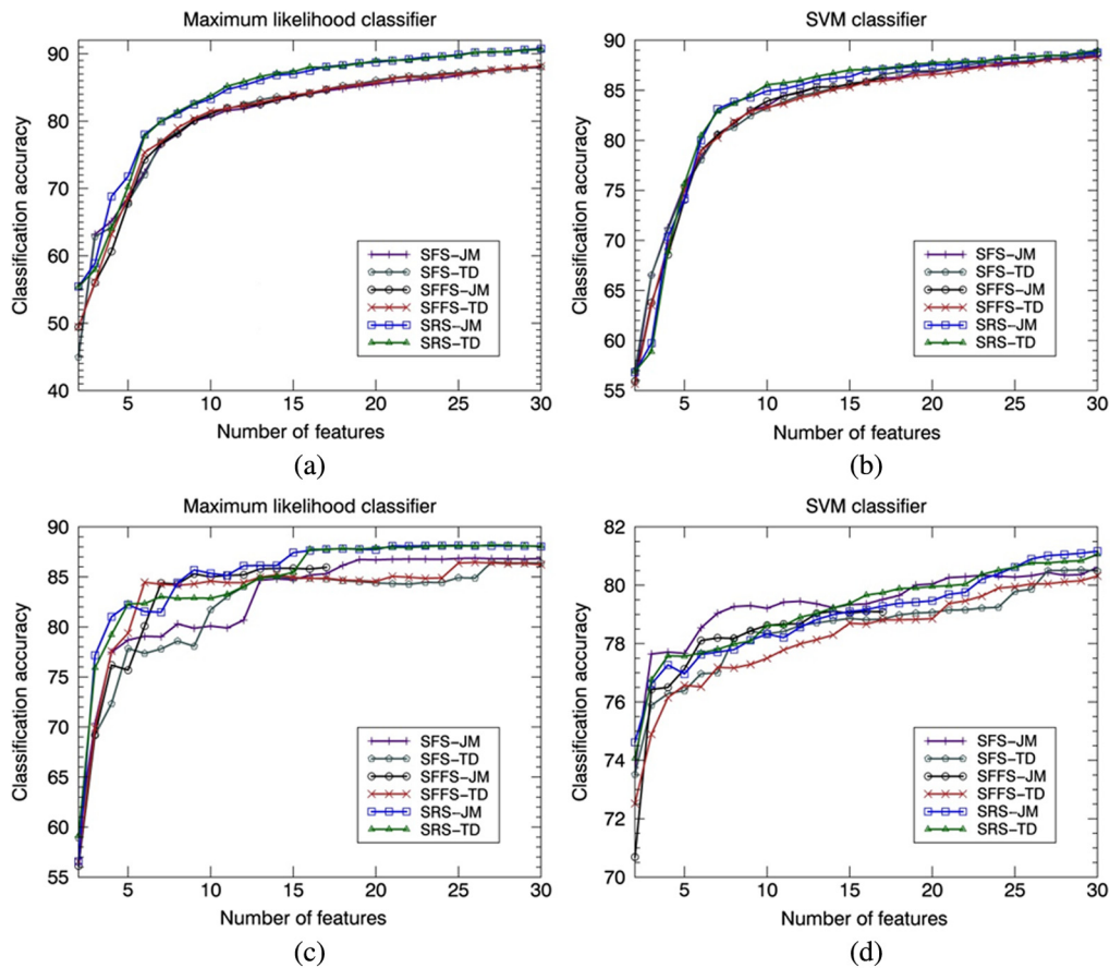
Fig. 10 The classification accuracy obtained with the classifiers MLC and SVM applied to the bands and channels identified by SRS, SFS, and SFFS using the JM and TD separability metrics; (a) and (b) Indian Pines and (c) and (d) Salinas scenes.
