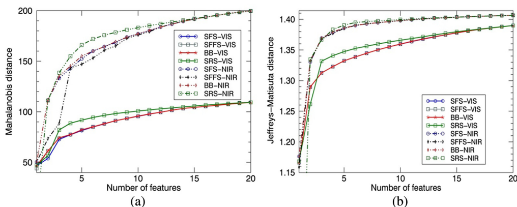
Fig. 6 The mean class separability versus the number of features obtained by applying the (a) Mh and (b) JM distances and the four algorithms described in the text; the datasets used are two spectral subsets with 20 channels of the Indian Pines scene from VIS and NIR spectral regions.
