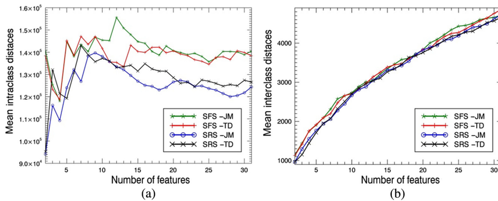
Fig. 9 The mean (a) intraclass and (b) interclass distance of 13 classes for the Indian Pine dataset with a different number of features when JM and TD measures are applied with the SRS and SFS search algorithms.
