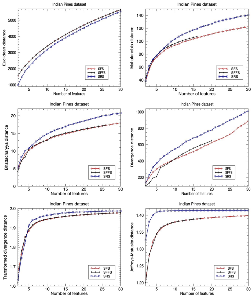
Fig. 7 The mean separability distance of the features obtained with different algorithms for the Indian Pines dataset.
