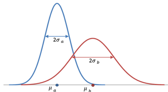
Fig. 1 Two hypothetical classes with normal distribution in one-dimensional feature space.
