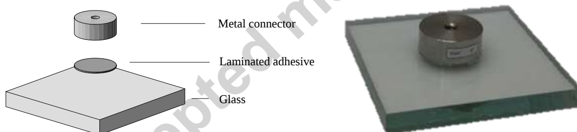
Figure 2: Scheme and photo of the specimen used in the tensile tests
