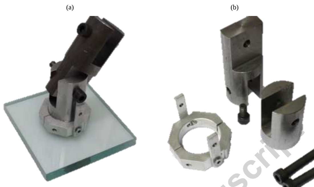
Figure 5: Photos of (a) a laminated connection with the metal fixture for LVDTs (b) exploded view
