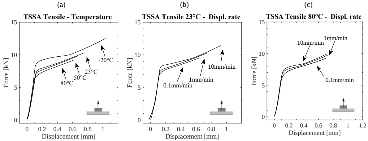
Figure 8: TSSA laminated connections under tensile force (a) Test results at -20°C, 23°C, 50°C and 80°C at 1mm/min (b) Test results at different displacement rates at 23°C (c) Test results at different displacement rates at 80°C
