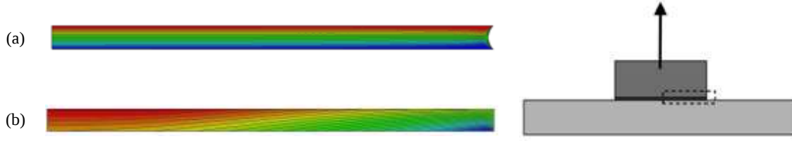
Figure 25: Distribution of the displacement field and deformation along z-direction of the adhesive from middle to perimeter (left to right) (a) soft adhesive (b) rigid adhesive
