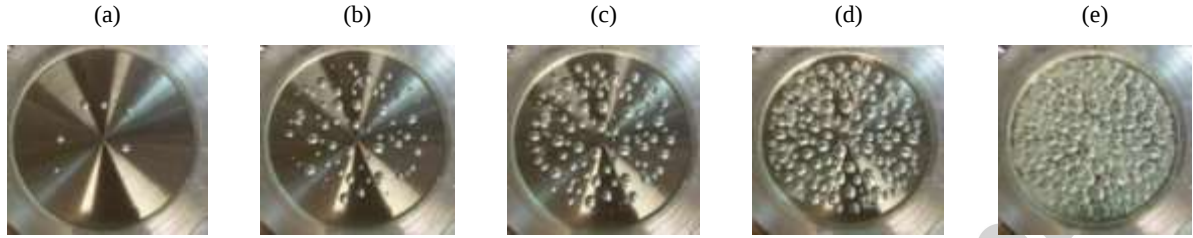
Figure 15: Evolution of cohesive bubble in SG laminated connection under tensile force (a) bubble formation (b-c) bubbles expand and new bubble are formed (d) distance between bubble is constant and number of bubble is stable (e) bubbles collapse and the remaining adhesive material form filaments that elongate
