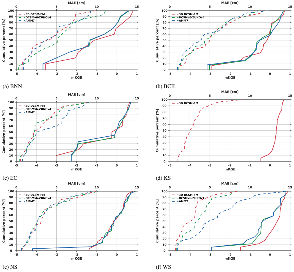
Figure 3.5: The cumulative distribution functions for both the MAE (dashed lines) and mKGE (solid lines) metrics per hydrodynamic model for all tide gauges located in the subregion.
