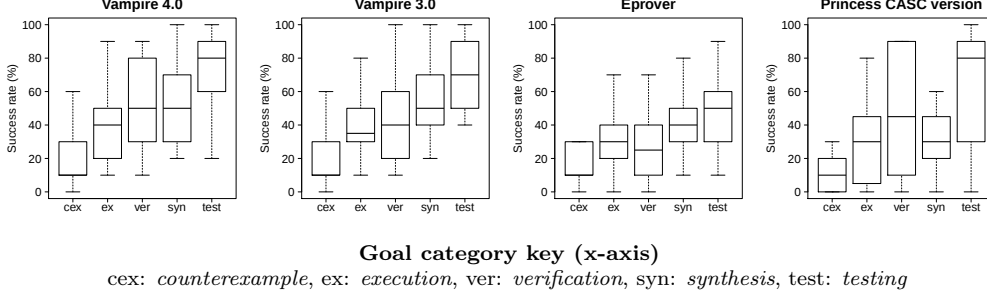
Figure 5: SQL + QL : Prover success rates greatly vary with compilation strategy (RQ1).
