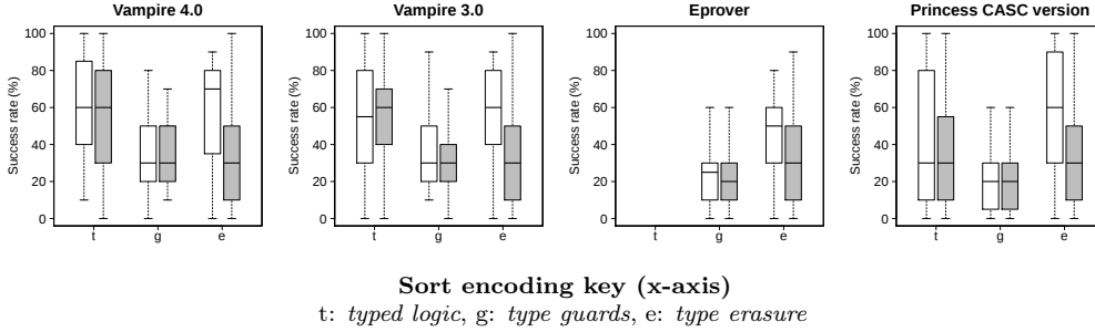
Figure 6: SQL (white) + QL (grey) : Using type guards for sort encoding significantly lowers prover performance (RQ2).
