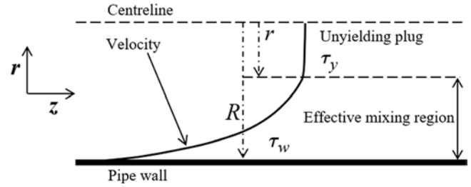
Figure 2 The velocity profile of a fluid with a non-zero yield stress inside a circular pipe
