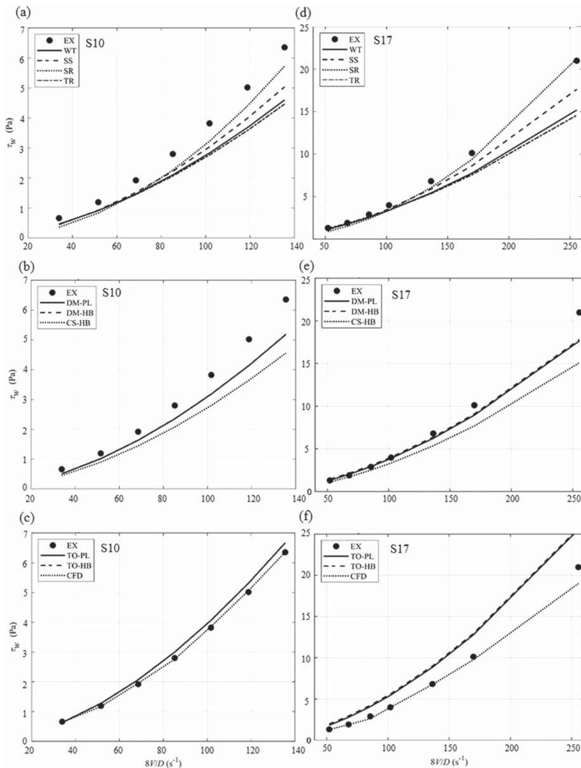
Figure 3 Shear stress vs. strain rate for S10 (left) and S17 (right). The graphs (a) & (d) correspond to the models WT, SS, SR & TR; (b) & (e) correspond to DM-PL, DM-HB & CS-HB and (c) & (f) correspond to TO-PL, TO-HB & CFD. In each graph, EX represents the experimental data points shown using solid black dots.
