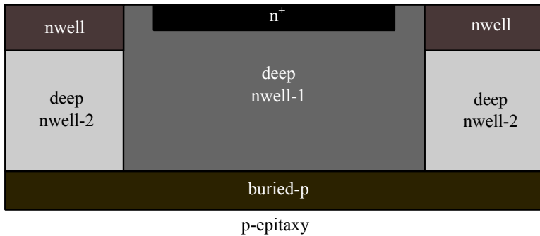
Figure 5.1: Electrical microlens: device cross section fabricated in 180nm CMOS technology.
