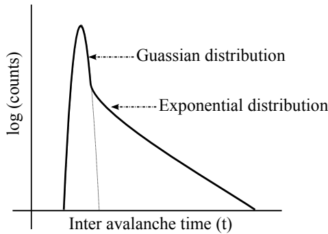
Figure 2.11: Statical distribution of photo-response of the SPAD.
