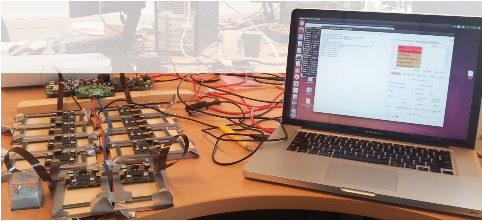
Figure 6.8: Prototype model comprising 10 DPCU nodes and 1 master snoopers node. DPCU was ported into Spartan-6 based FPGA boards that are custom designed for SPADnet photonic module. Snooper was ported on to ML605 board from Xilinx Inc.
