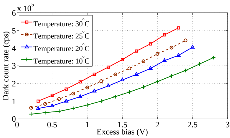
Figure 5.5: Electrical microlens: DCR characterization performed at various temperatures with the dead time tuned to 10\mu s .
