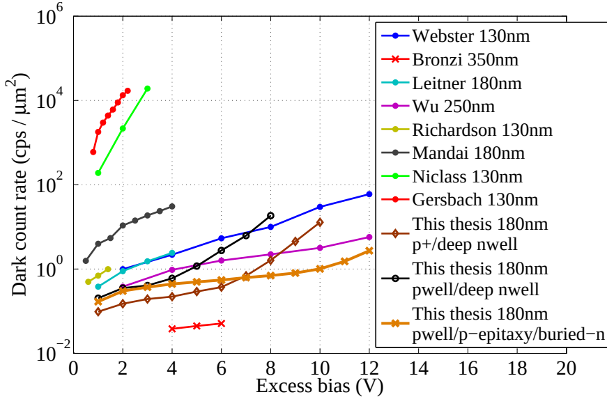
Figure 3.32: pwell-2/p-epitaxy/buried-n SPAD: state-of-the-art DCR comparison.
