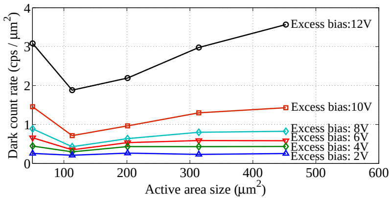
Figure 4.11: DCR normalized with respect to the active area for devices designed with different curvatures. Each measurement point is the mean DCR obtained from 4 devices when the dead time was tuned to 400ns.
