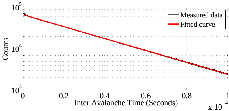
Figure 3.25: pwell-1/p-epitaxy/buried-n SPAD: afterpulsing probability measurement results at 10V excess bias, performed with a deadtime of 300ns.
