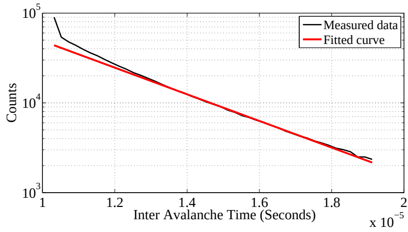
Figure 5.6: Electrical microlens: afterpulsing probability measurement results at 2V excess bias, performed with the device deadtime configured to 10\mu s .
