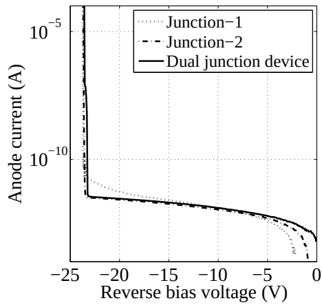
Figure 5.10: Dual junction SPAD: breakdown voltage measurement.
