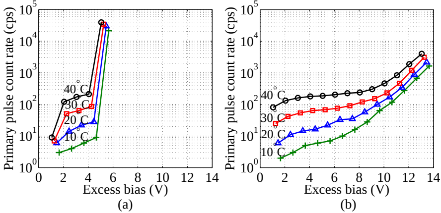
Figure 4.6: DCR characterization performed at various temperatures with the dead time tuned to 10\mu\text{s} : (a) design-1, (b) design-2.
