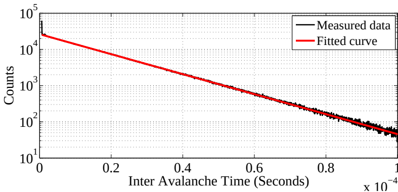
Figure 3.18: pwell/deep nwell SPAD: afterpulsing probability measurement results at 10V excess bias, performed with the device deadtime configured to 300ns.
