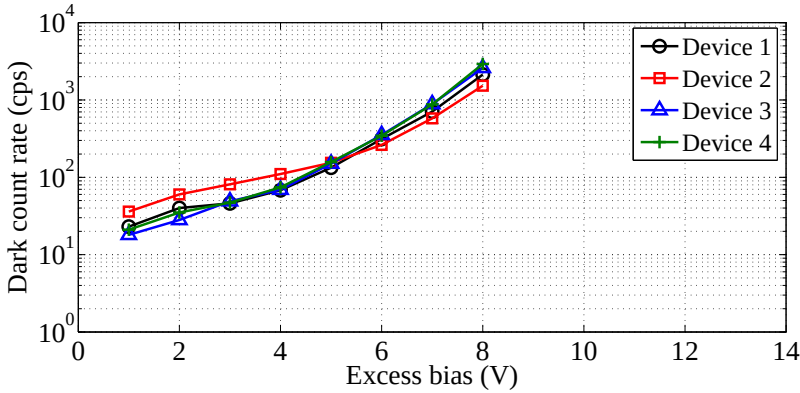
Figure 3.17: pwell/deep nwell SPAD: DCR characterization for four devices with the dead time tuned to 300ns.
