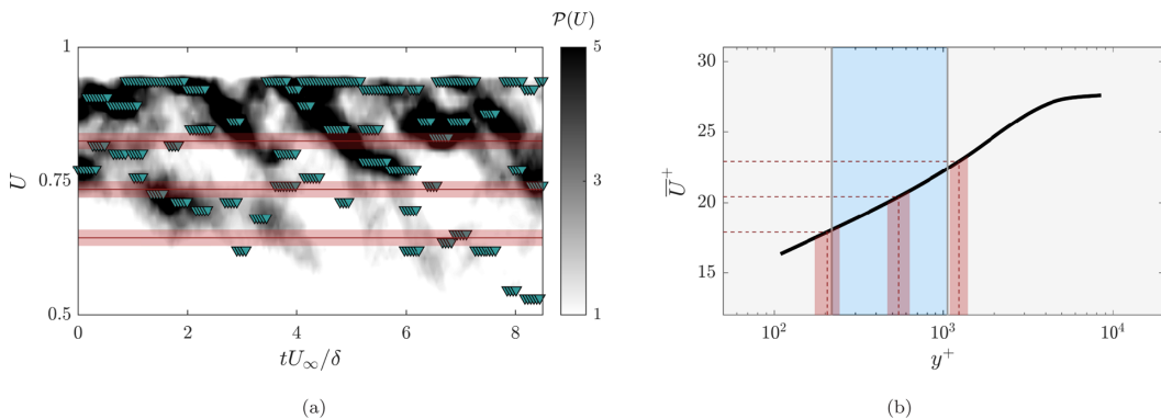
FIG. 8. (a) Illustration of multiple time-coherent UMZ peaks (symbols) overlaid on \mathcal{P}_U . Statistics of \mathcal{T}(U_m) in what follows are calculated at 0.63 \leq U_m/U_\infty \leq 0.66 , 0.72 \leq U_m/U_\infty \leq 0.75 , and 0.81 \leq U_m/U_\infty \leq 0.84 (shaded regions). (b) Corresponding wall-normal locations for the selected velocity regions in (b), based on the mean, \bar{U} (here for TRPIV). Blue shaded region indicates the logarithmic region extent ( 3/\sqrt{\text{Re}_\tau} \leq y/\delta \leq 0.2 ).
