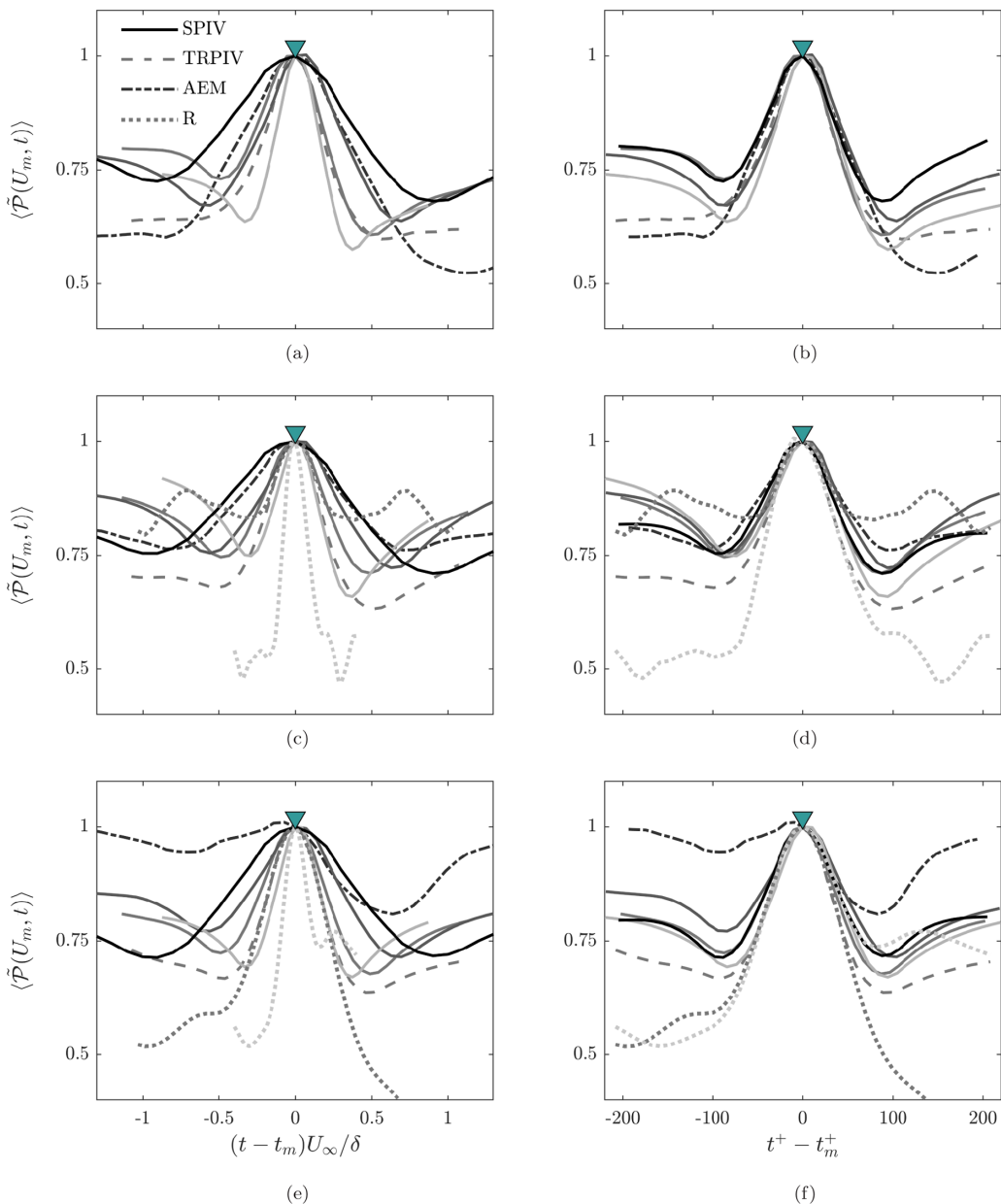
FIG. 9. Conditionally averaged PDF values with respect to time, \langle \tilde{\mathcal{P}}(U_m, t) \rangle , for all data sets, normalised with the maximum peak value, \mathcal{P}(U_m, t_m) . Temporal axis in outer (left) and inner (right) scaling, for 0.63 \leq U_m/U_\infty \leq 0.66 (a), (b); 0.72 \leq U_m/U_\infty \leq 0.75 (c), (d); and 0.81 \leq U_m/U_\infty \leq 0.84 (e), (f). Increasing Re_\tau is denoted with lighter colors. Following Fig. 8(a), symbols denote the UMZ peaks at t = 0 .
