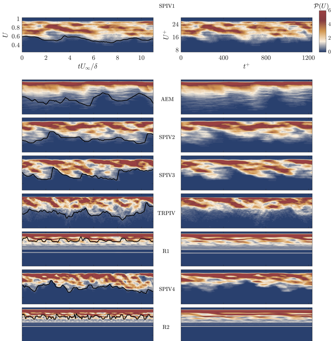
FIG. 2. Variation of \mathcal{P}(U) over time in increasing \text{Re}_\tau from top to bottom. Matching temporal extent in outer (left) and inner (right) units. Black solid lines denote U_* = \min(U | \mathcal{P}(U, t) > \mathcal{P}_{\text{th}}) .
