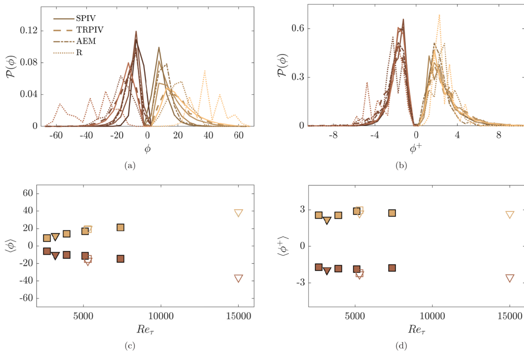
FIG. 4. Probability density function and mean values of transition angles \phi_+ and \phi_- , in outer (a), (c) and inner (b), (d) scaling ( \phi = \tan^{-1}(\Delta U_*/\Delta t) ). SIV is denoted by \blacksquare , AEM by \blacktriangledown , TRPIV by \square , and R1 (R2) by \nabla (see also Table I). Colors of each transition angle as in Fig. 3 (with lighter shades indicating increasing Re_\tau ).
