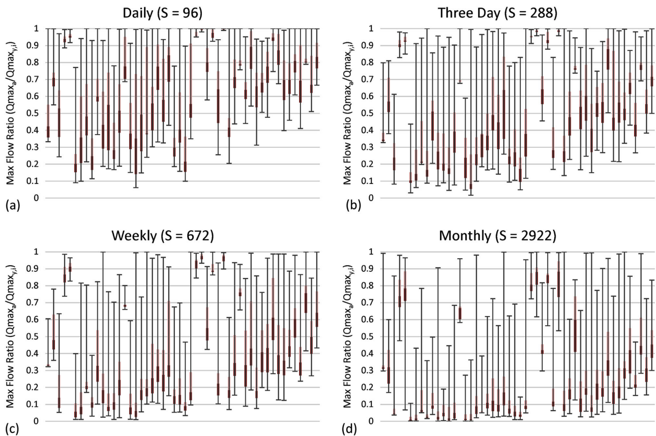
Fig. 5 Maximum flow ratio between maximum flow calculated from subsampled data for each gauging station ( y ) and iteration ( i ) (i.e., Q_{max_{y,i}} ) and actual maximum flow from the 15-min record (i.e., Q_{max_a} ) expressed as a fraction (i.e., Q_{max_{y,i}}/Q_{max_a} ). All maximum flow ratios were calculated for the 7-year period from 2008 to 2014. Data for all four subsample intervals are shown. Each plot contains the median (Q2; interface between light red and dark red ), the 1st and 3rd
