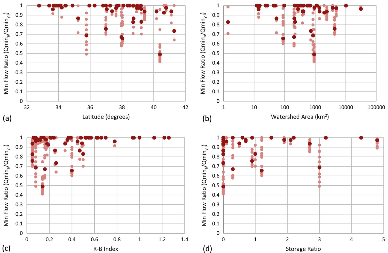
Fig. 10 Scatter plots of minimum flow ratio as a function of a Latitude (decimal degrees), b watershed area ( \text{km}^2 ), c Richards-Baker flashiness index (R-B Index), and d storage ratio. Average data for all 50 sites shown in dark red ; data for all 50 iterations shown in light red .
