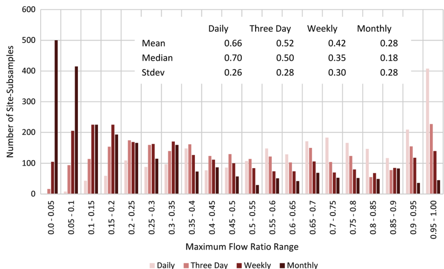
Fig. 5 Maximum flow ratio between maximum flow calculated from subsampled data for each gauging station ( y ) and iteration ( i ) (i.e., Q_{max_{y,i}} ) and actual maximum flow from the 15-min record (i.e., Q_{max_a} ) expressed as a fraction (i.e., Q_{max_{y,i}}/Q_{max_a} ). All maximum flow ratios were calculated for the 7-year period from 2008 to 2014. Data for all four subsample intervals are shown. Each plot contains the median (Q2; interface between light red and dark red ), the 1st and 3rd
