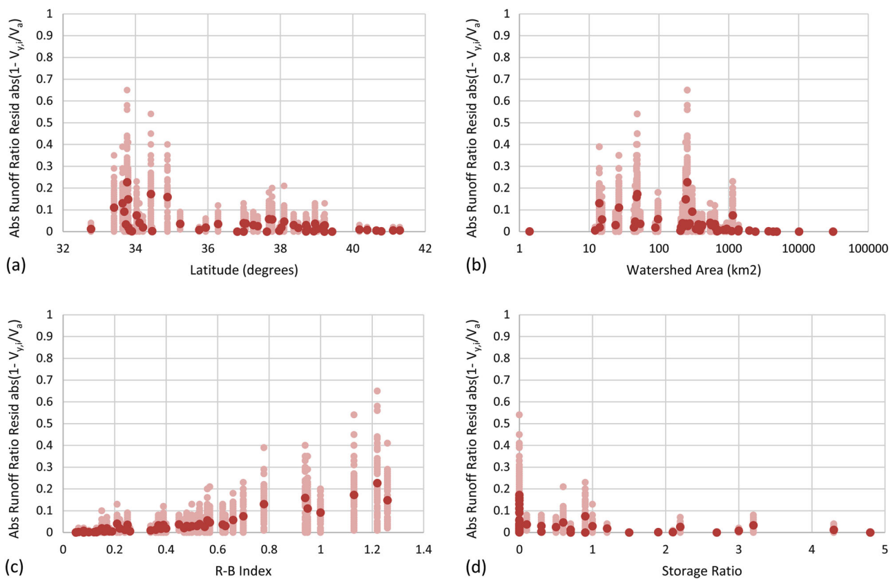
Fig. 12 Scatter plots of the absolute value of the runoff ratio residual (i.e., 1 - V_{y,i}/V_a ) as a function of a latitude (decimal degrees), b watershed area ( \text{km}^2 ), c Richards-Baker flashiness index (R-B Index), and d storage ratio. Average data for all 50 sites shown in dark
