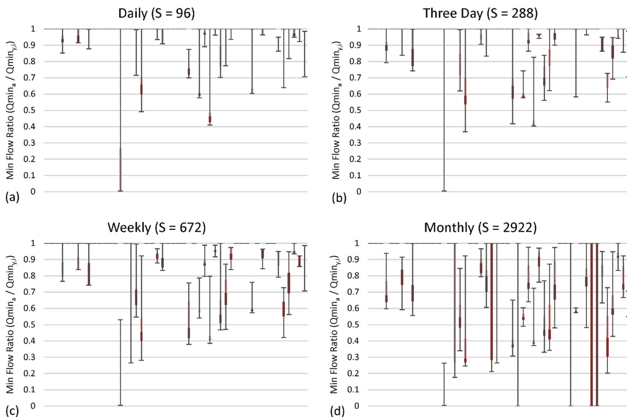
Fig. 3 Minimum flow ratio between actual minimum flow from the 15-min record (i.e., Q_{min,a} ) and minimum flow calculated from subsampled data for each gauging station ( y ) and iteration ( i ) (i.e., Q_{min,y,i} ) and expressed as a fraction (i.e., Q_{min,a}/Q_{min,y,i} ). All minimum flow ratios were calculated for the 7-year period from 2008 to 2014. Data for all four subsample intervals are shown starting from the top left . Each plot contains the median (Q2; interface between light and dark red ), the 1st and 3rd quartiles (Q1 and Q3; bottom of dark red
