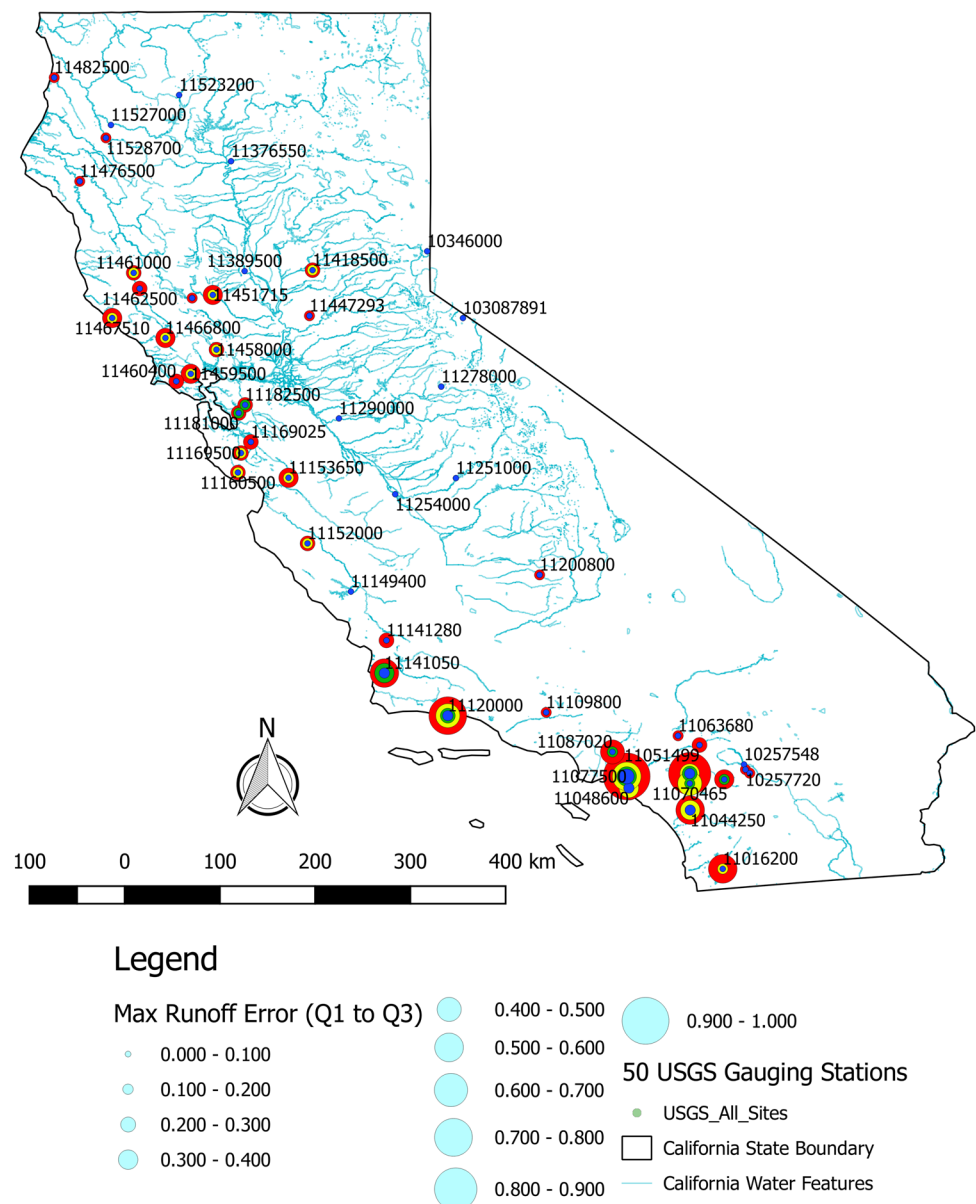
Fig. 9 Map figure of 50 USGS stream gauges labeled with USGS Station ID. At each location, there are four concentric and scaled circles. The circles are scaled by maximum runoff error (i.e., maximum of the runoff ratio residuals) within the 1st and 3rd quartiles from the 50 subsample iterations. Daily, three day, weekly, and monthly subsample intervals are shown in blue, green, yellow, and red, respectively
