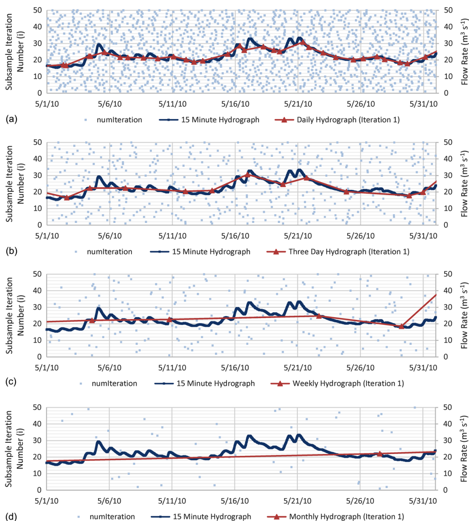
Fig. 2 Example bootstrap randomized subsamples with replacement for each of the 50 iterations ( light blue dots ), original 15-min hydrograph ( dark blue ), and hydrograph from subsample iteration 1 ( red ) for the Truckee River near Farad. The horizontal axis displays time, in this case the month of May from 2010. The primary (left) vertical axis displays subsample iteration number ( i ), and the secondary (right) vertical axis displays flow rate. Each horizontal gridline represents a single subsample iteration from 1 to 50. Each light blue square on the horizontal gridlines represents a date time selected for the respective subsample iteration. The 30 subsamples that make up the hydrograph for iteration 1 shown as red triangles coincide horizontally, that is with respect to time, with the 30 light blue squares on the first horizontal gridline above the x-axis (i.e., subsample iteration number 1). The data shown are for a daily, b three day, c weekly, and d monthly subsample intervals
