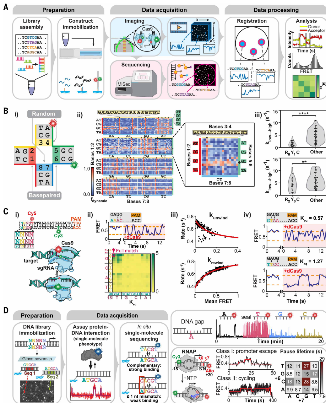
Fig. 3. Quantitative insights from multiplexed single-molecule platforms reveal sequence-dependent variation in kinetic and thermodynamic behavior. (A) Overview of a MUSCLE or SPARXS experiment (the example shown here is Cas9 DNA unwinding). A DNA sequence library is synthesized and immobilized on a flow cell. Single-molecule fluorescence imaging yields time traces from individual molecules. The same flow cell undergoes NGS to identify the sequence and spatial position of each DNA cluster. Fluorescence and sequencing data are aligned to extract kinetic or equilibrium parameters, such as FRET states or transitions, per sequence. [Adapted with permission from Elsevier (9); adapted with permission from (71); adapted with permission from Springer Nature (76)] (B) Sequence-dependent Holliday junction dynamics in a 4096-member SPARXS library. (i) Bases 3, 4, 7, and 8 are randomized. (ii) Heatmap of the dynamic molecule fraction across variants, with clustering seen at bases 7:8. Stars indicate fully matched junctions. (iii) Transition rates are reduced in sequences with the RYC motif. [Adapted with permission from (72)] (C) Cas9 unwinding and cleavage dynamics using MUSCLE. (i) smFRET assay with a DNA library varying four PAM-distal bases. (ii) FRET traces for a mismatched sequence (top) and equilibrium constants for all sequences (bottom), organized by identity at positions 17 to 20. (iii) Unwinding-rewinding rates plotted versus mean FRET, with model fits. (iv) FRET traces and cleavage for selected mismatched sequences show impaired cleavage correlating with FRET, linking kinetics to outcomes. [Adapted with permission from (71)] (D) SPIN-seq. (Left) Immobilized DNA libraries are imaged for biomolecular interactions (e.g., protein binding kinetics), denatured, and rehybridized. Sequence is read by hybridizing fluorescent “seals” to gapped DNA; seal binding distinguishes complementary from mismatched sequences. (Top right) Sequential interrogation of a DNA gap by four seals, with T-seal as the match. (Bottom right) smFRET monitoring of transcription initiation reveals distinct promoter DNA pathways and measures pause lifetimes across a 16-sequence library (+6/+7 degenerate bases). [Adapted from (44), CC BY 4.0; adapted from (73), CC BY 4.0]
