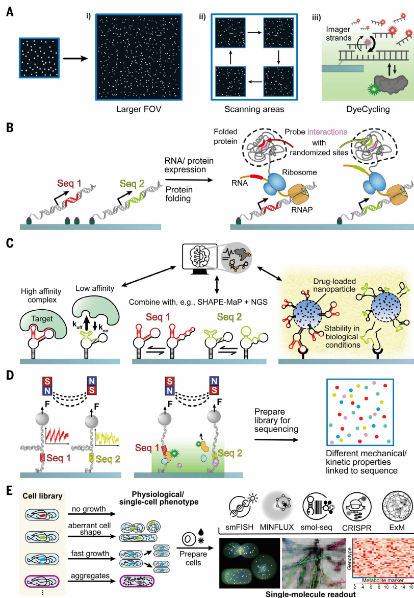
Fig. 4. Expanding multiplexed single-molecule analysis across molecular scales and applications. (A) Increasing data collection efficiency. Throughput can be maximized by (i) using full CMOS camera fields of view or (ii) cycling through multiple FOVs sequentially for slower kinetic processes. (iii) DyeCycling (81) sustains donor fluorescence in single-molecule FRET by continuously exchanging photobleached dyes during TIRF excitation, enabling longer observation windows for kinetic analysis and increasing the statistical power of equilibrium binding measurements from fewer molecules. (B) Peptide and protein libraries. DNA-barcoded peptide and protein libraries allow single-molecule kinetic screening of binding, folding, or enzymatic activity. Techniques such as ribosome and cDNA display link behavior to sequence, enabling functional profiling across millions of variants. Applications span signaling, immunity, and protein engineering. (C) Aptamer characterization. High-throughput screening of nucleic acid aptamers at the single-molecule level can uncover folding pathways, binding kinetics, and structural dynamics tied to sequence. This enables identification of aptamers with high specificity, adaptability, and functional stability for therapeutic, diagnostic, and analytical uses. (D) Sequence multiplexing in other single-molecule methods, such as magnetic tweezers. Incorporating sequence-encoded tethers enables parallel force spectroscopy on multiple DNA or RNA constructs, facilitating comparison of mechanical responses or enzymatic processing. These platforms can also include colocalization-based fluorescence readouts for monitoring protein dynamics or substrate conformational changes alongside mechanical data. (E) Expansion to cell libraries. Linking single-molecule readouts to cell-based assays involves using genetically defined cell libraries combined with phenotypic sorting (e.g., growth, stress). Cells can be analyzed for molecular structure, localization, and dynamics using FRET, MINFLUX (128), expansion microscopy (129), and smFISH (130,131), connecting genotype, phenotype, and mechanism in a unified experimental pipeline. Visual examples are stylized illustrations inspired by reported single-molecule observations in cells.
