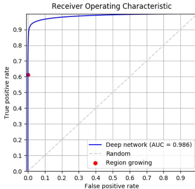
Figure 2: Receiver Operating Characteristic for the segmentation of both ventricles. Please note that the region growing algorithm is represented by a single point as the mentioned method is not probabilistic in contrast to the deep network.
