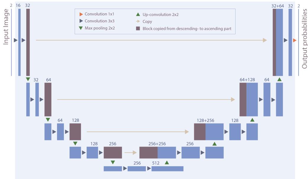
Figure 1: The fully convolutional network used for training our model. This is a U-net-like architecture 16,17 with slight modifications as described in the text.
