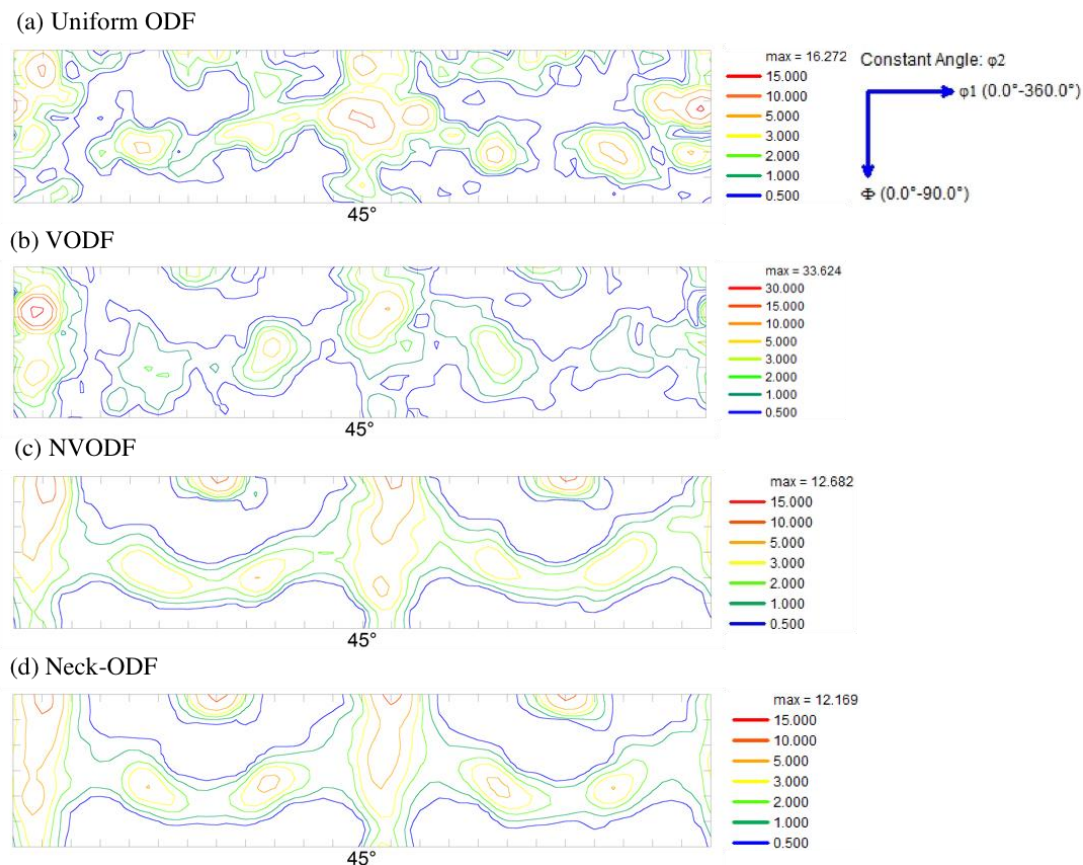
Figure 4. \phi_2=45^\circ section of ODFs of the material at two different deformation levels; (a) Uniform deformation UODF (calculated from 796000 data points), (b) post uniform VODF (131000 data points), (c) post uniform NVODF (460000 data points) and (d) Necking or post uniform ODF consist of the merged ODFs in b and c.
