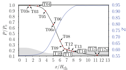
Fig. 4. Static pressures measured along the nozzle during the PR.028-NT.001 experimental run together with the related total expanded uncertainty bars, see Table 2. The pressure is non dimensionalized with the average value of the total pressure at the inlet P_0 = 18.36 bara and the axial coordinate with the throat height H_{th} = 7.73 mm. Static pressures resulting from the Euler simulation ( - ) and exp. results ( x ). The centerline compressibility factor ( - - ) is calculated with the PR eqn. of state.
