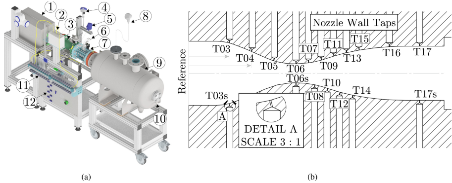
Fig. 1. The primary components and instrumentation of the nozzle TS. (a). ①: Flow Meter KROHNE OPTIMASS 6400 F F – Tag FT0004; ②: Scanivalve DSA3218; ③: Settling Chamber; ④: WIKA UPT 20 – Tag PT011; ⑤: WIKA TR10-C PT100 – Tag TT015; ⑥: Taps; ⑦: Nozzle Housing; ⑧: WIKA UPT 20 – Tag PT014; ⑨: Receiver; ⑩: WIKA TR10-C PT100 – Tag TT014; ⑪: Liquid Trap; ⑫: Scanivalve Control Panel. (b). A cross-section of the planar nozzle showing the positioning of the eighteen pressure taps. Three taps are symmetrically aligned and are indicated by the letter s. Detail A shows that the opening of each tap is perpendicular to the nozzle profile wall. Distances to taps from Reference in [mm]: T03(s) = 15.96; T04 = 24.72; T05 = 33.55; T06(s) = 42.4; T07 = 47.44; T08 = 49.9; T09 = 52.57; T10 = 55.01; T11 = 57.5; T12 = 59.91; T13 = 62.53; T14 = 64.89; T15 = 67.47; T16 = 79.35; T17(s) = 91.3. Two taps, T01 & T02, are located in the settling chamber at the first and second flange. Nozzle profile designed for the MM working fluid at the design conditions: T_0 = 252^\circ\text{C} , P_0 = 18.4 bar and a back pressure of 2.1 bar with a throat height H_{th} = 7.5 mm. See Nozzle B in [5, App. B] for the geometric points defining the profile. Fluid properties estimated with the multi-parameter equation of state available in the thermophysical property database of NIST [8].
