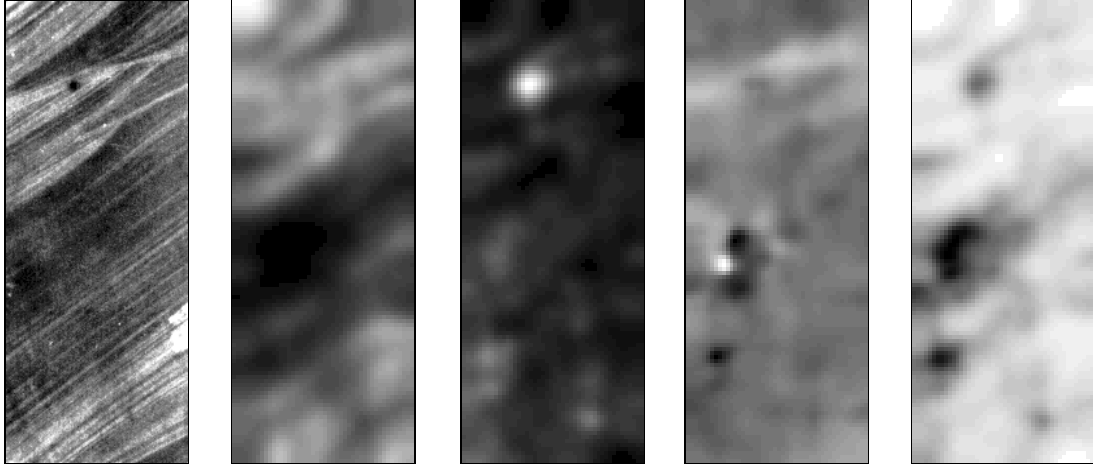
Figure 4: Gradient-square tensor method applied to a region of low SNR. In the middle-left part of the image the noise dominates the gradient-square tensor producing an unreliable estimate of local orientation. a) input image; b) largest eigenvalue \lambda_1 ; c) smallest eigenvalue \lambda_2 ; d) local orientation \varphi ; e) anisotropy (1-\lambda_2/\lambda_1) .
