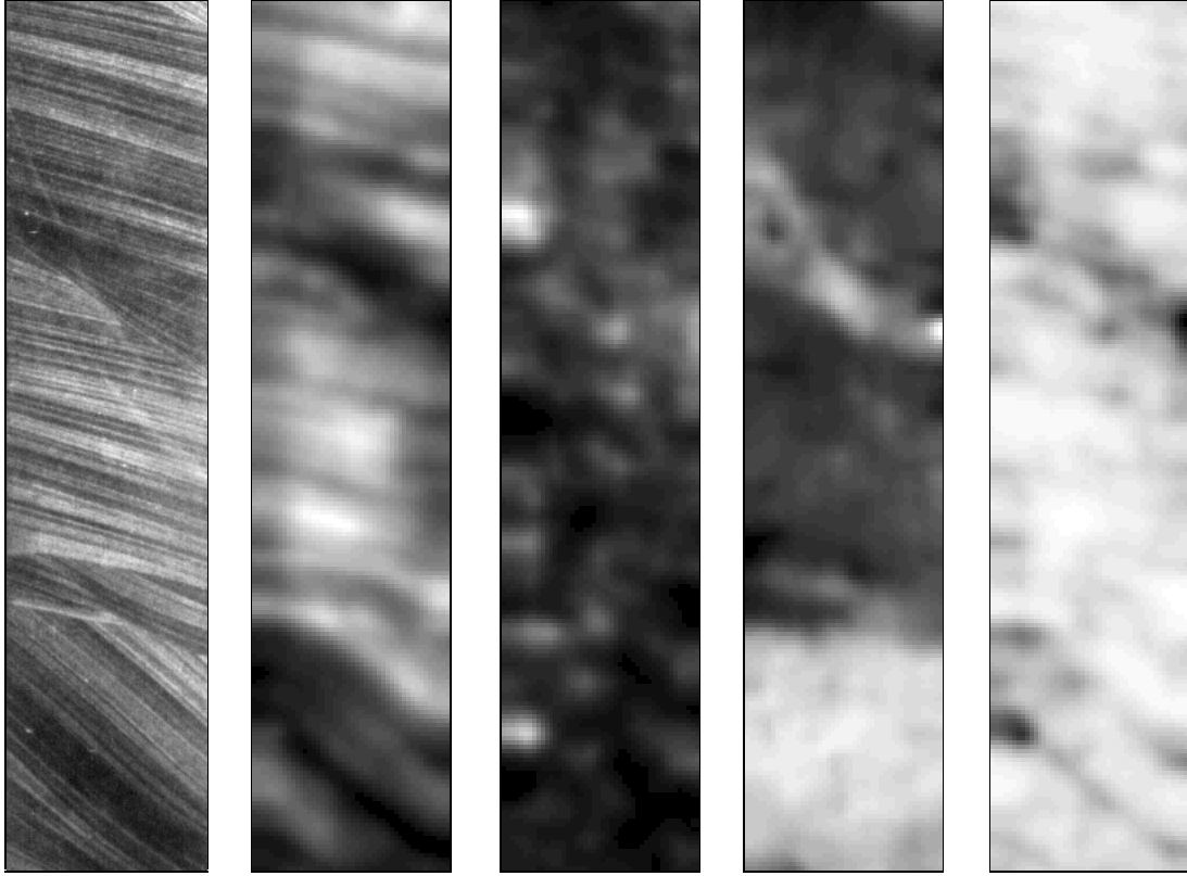
a) b) [0, 1.5] c) [0, 0.3] d) [0.2, 0.9] e) [0.4, 1] Figure 3: A smoothed gradient-square tensor yields the following information. a) input image; b) largest eigenvalue \lambda_1 ; c) smallest eigenvalue \lambda_2 ; d) local orientation \phi ; e) anisotropy (1-\lambda_2/\lambda_1) .
