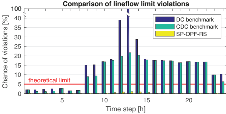
Figure 4.4: Empirical violation level of lineflow limit for different formulations for the IEEE 30-bus benchmark case study.
