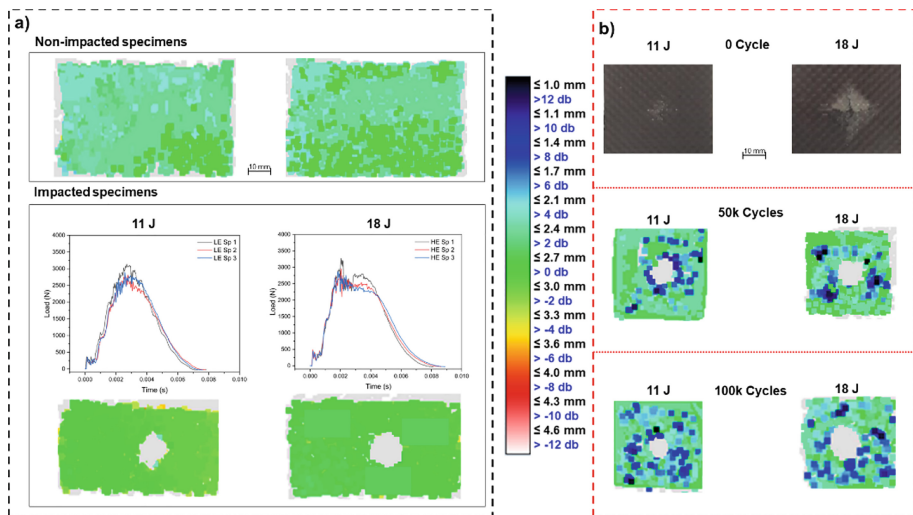
Fig. 2. Mechanical test analysis: a) impact test curve and C-scan images, and b) propagation of interlaminar fatigue damage (C-scan images).
