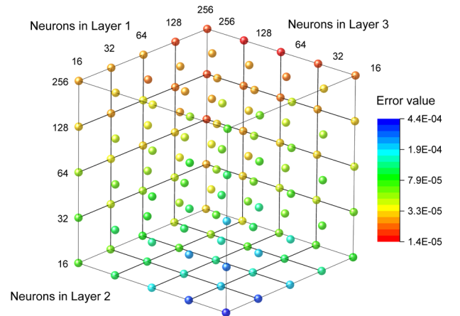
(b) Predictions error with three hidden layers model
