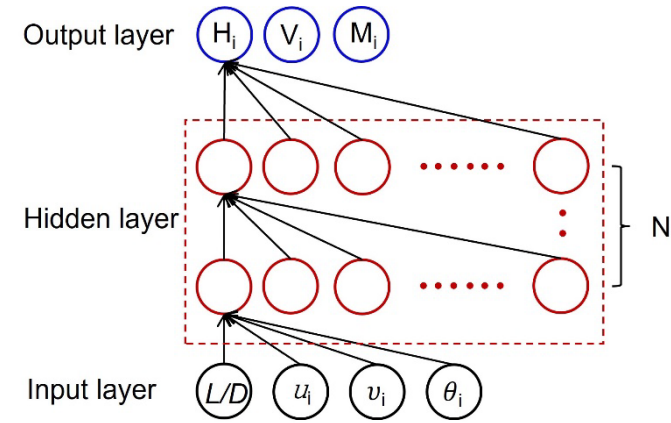
Figure 3 Fully connected neural network
