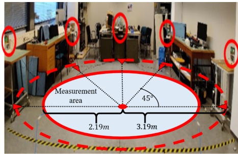
(b) Laboratory radar layout with 5 nodes.
