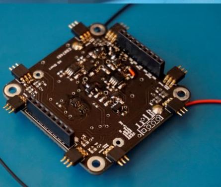
Figure 10 Battery board and EPS board
