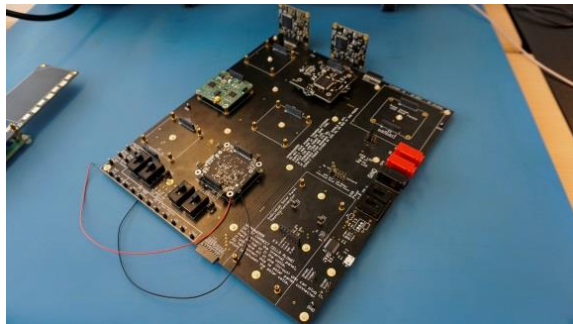
Figure 17 Delfi-PQ FlatSat
