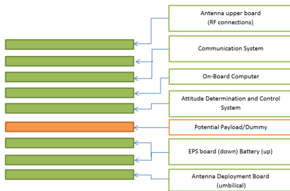
Figure 15 Satellite configuration
