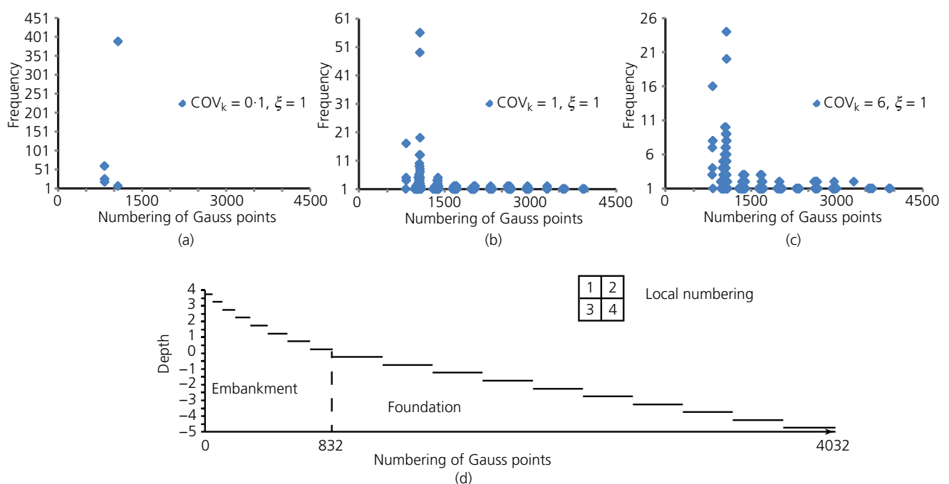
Figure 16. Frequency and locations of Gauss points with v_{\max} for different \text{COV}_k values
