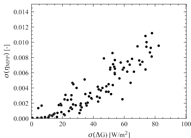
Figure 2. Daily dispersion of differences in irradiance, \sigma(\Delta G) , causes increased daily dispersion of the calculated efficiency, \sigma(\eta_{MPP}) , for 100 randomly selected days. Two outliers were removed for clarity.
