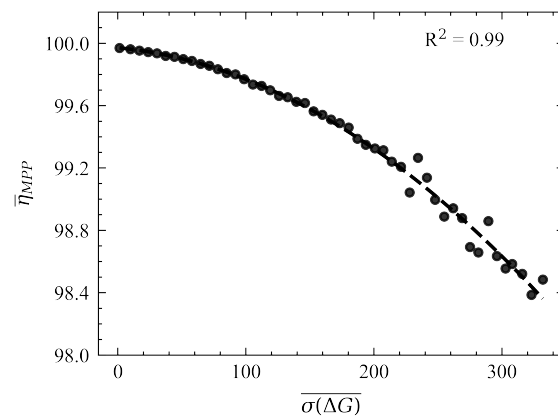
Figure 3. Drop of the binned average efficiency, \bar{\eta}_{MPP} , of the P&O algorithm as a function of the mean irradiance variability in each bin, \sigma(\Delta G) . The coefficient of determination ( R^2 ) is included in the graph to indicate the goodness of fit. Other variability metrics can also be fitted with the model. The fitting parameters are given in Appendix A.
