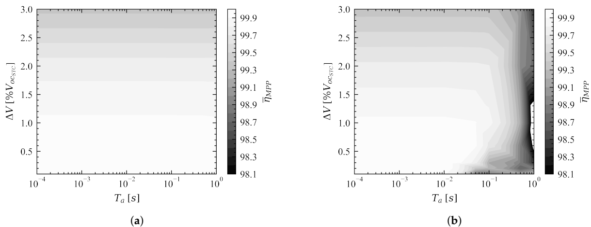
Figure 4. Sensitivity of the P&O algorithm efficiency, \eta_{MPP} , to its parameters under (a) clear skies, and (b) variable irradiance.
