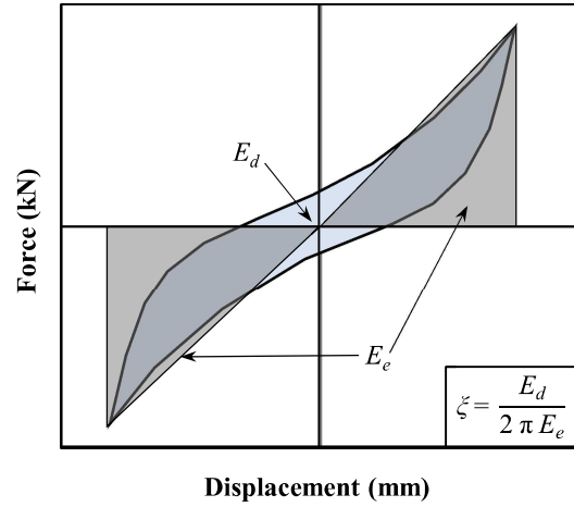
Figure 4: Determination of the equivalent damping ratio from the energy dissipated in one full cycle and the corresponding elastic energy
