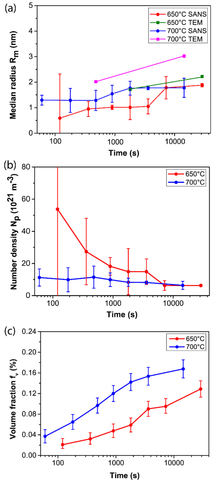
Fig. 8. Evolution of precipitate (a) median radius R_m , (b) number density N_p , (c) volume fraction f_v as derived from SANS measurements of samples annealed at 650 °C and 700 °C. The R_m values, especially for the 650 °C 8 h, 700 °C 1 h and 700 °C 4 h samples are underestimated due to the big (Ti,V)C precipitates on grain boundaries not properly captured in the fits at low Q values in Fig. 7c and d.
