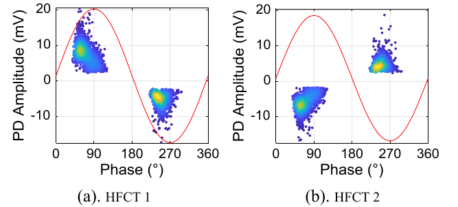
Fig. 12. PRPD patterns of partial discharges at 108 kV rms .
