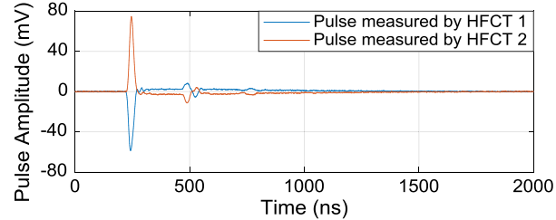
(c). Pulse simulated from the cable joint between two HFCTs.
