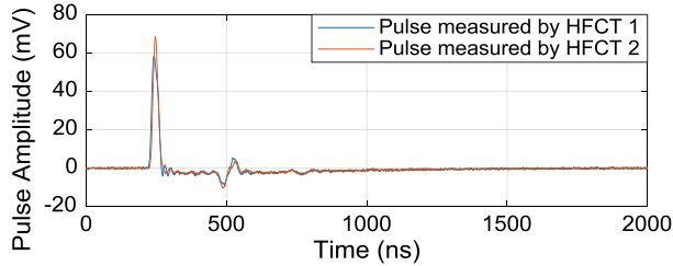
(a). Pulse injected from termination 1.
