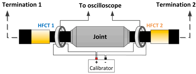
Fig. 8. Pulses simulated from the cable joint.
