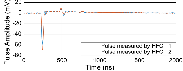
(b). Pulse injected from termination 2.
