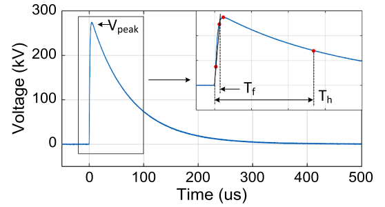
(a). Test voltage waveform of impulse voltage.
