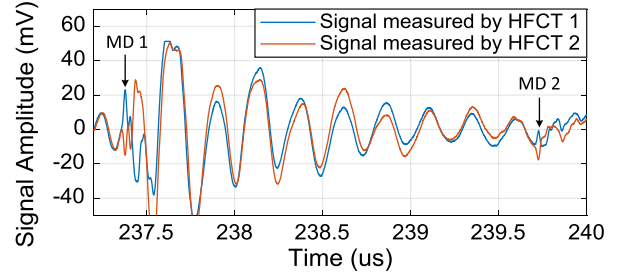
(a). TRPD pulses of MD1 and MD2 measured under impulse voltage.
