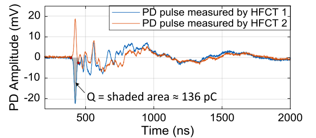
(a). TRPD pulses of one partial discharge at negative cycle of 108 kV rms .
