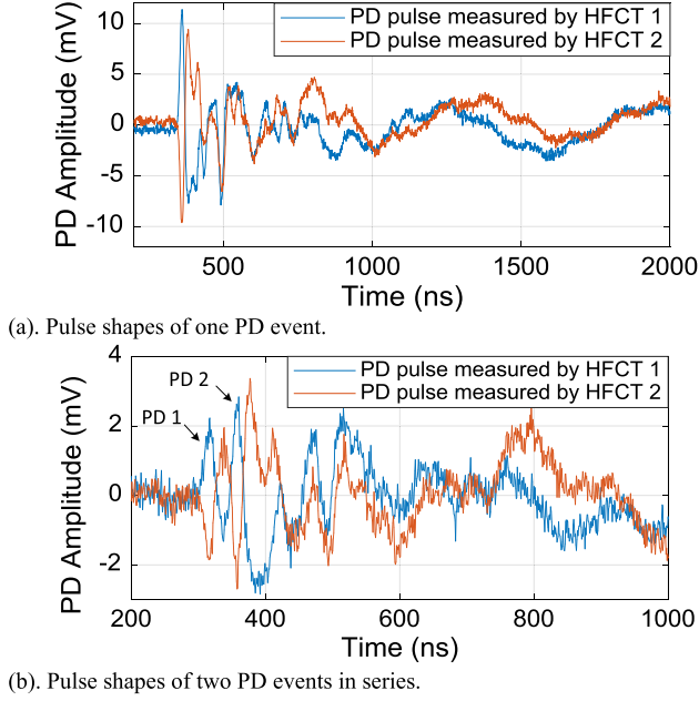
Fig. 25. TRPD patterns of partial discharges from cable joint measured with filter A + B.
