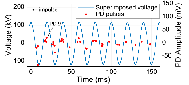
(b). PD occurrence during the first eight cycles after the impulse.
