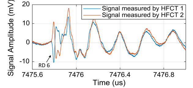
(b). TRPD pulses of RD6 measured under impulse voltage.
