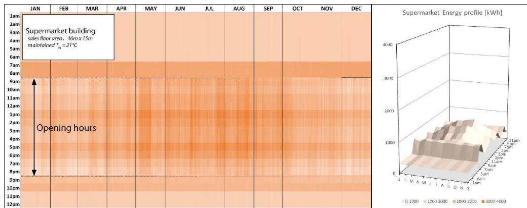
Figure 5.3b. Supermarket energy balance: The supermarket has a year-round cooling demand, ranging from 2 kW in winter up to 40 kW during peaks in summer. The building does not have a heating demand at any moment of the year.
