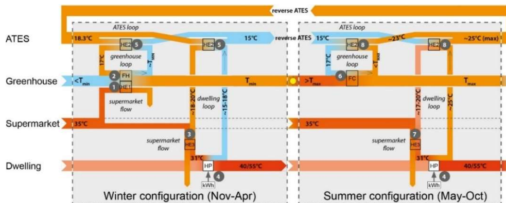
Figure 5.5. Abstract representation of the thermal energy flows in scenario 2a–d: the local system. Relevant medium/component temperatures are mentioned where ~ indicates an estimated temperature. FH = floor heating, FC = floor cooling, HE = heat exchanger. The ATEs reverses at the beginning of May, when the cooling season starts and at the end of October, when the heating season starts. The temperature of the warm well of the ATEs is assumed to drop with 3^{\circ}\text{C} between seasons (see section 5.2.5.3).
