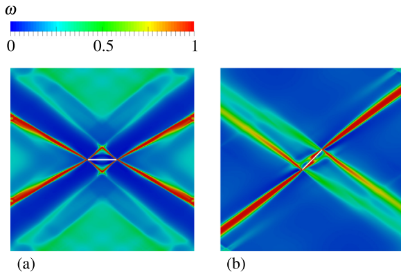
Fig. 9. Localization of damage, parameter \omega defined by Eq. (15), in a specimen subject to tensile stretching with an embedded rigid line inclusion inclined at angles \bar{\theta} = 0^\circ (a) and \bar{\theta} = 45^\circ (b) with respect to the horizontal axis. Shear bands exhibit a double symmetry in (a), while the shear bands closer to the inclusion axis are the most intense in (b).
