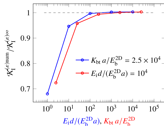
Fig. 3. Convergence of the mode I stress intensity factor evaluated numerically to that estimated analytically. The two values are calculated with reference to the two boundary value problems depicted in Fig. 2 on the right (for L = 10a ) and on the left, respectively. The numerical solution differs from the theoretical prediction by less than 1% when E_i d / (E_b^{2D} a) > 100 (blue line, with K_{bt} a / E_b^{2D} = 2.5 \times 10^4 ) or when K_{bt} a / E_b^{2D} > 250 (red line, with E_i d / (E_b^{2D} a) = 10^4 ).
