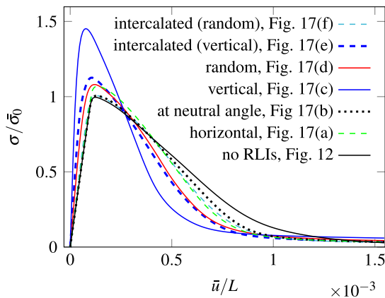
Fig. 18. Influence of RLIs' distributions on the global stress/strain response for the square samples analyzed in Fig. 17. A stress normalization is introduced through division by the maximum stress \sigma_0 referred to the sample without RLIs.
