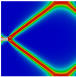
Fig. 12. Map of damage field \omega revealing shear bands as nucleated from an imperfection symmetrically placed along the left-hand boundary of the specimen (where RLIs are not present). The shear bands are inclined at the conjugate angles of \theta_{sb}^{(\pm)} \approx \pm 37^\circ with respect to the x -axis. The color scale is the same as in Fig. 9.
