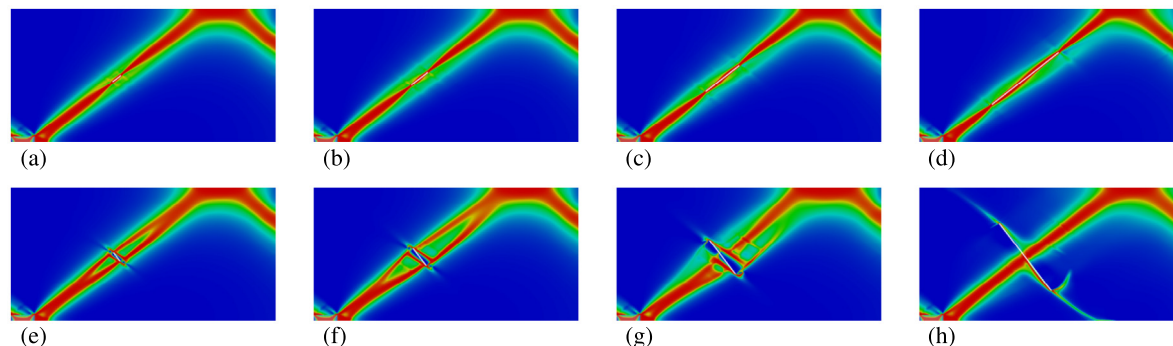
Fig. 14. Maps of damage field \omega revealing interaction of the shear bands nucleated from an imperfection with two symmetric RLIs of different lengths and at different inclinations. Due to symmetry, only the upper half of domain is reported. The color scale is the same as in Fig. 9.
