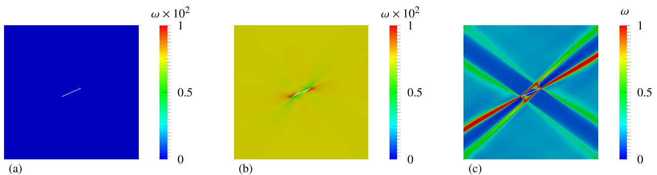
Fig. 10. Evolution of the damage field \omega in a specimen containing a single inclusion, inclined at the angle \bar{\theta} = \bar{\theta}_n \approx 24.09^\circ and corresponding to elastic neutrality: (a) the elastic state is unaffected by the inclusion up to just before damage initiation ( \bar{u}_y = 0.065\bar{U} ); (b) inelastic strain initiates damage concentration at the tips of the inclusion after damage initiation ( \bar{u}_y = 0.085\bar{U} ); and (c) a complex shear band pattern has emerged at the final imposed displacement \bar{u}_y = \bar{U} .
