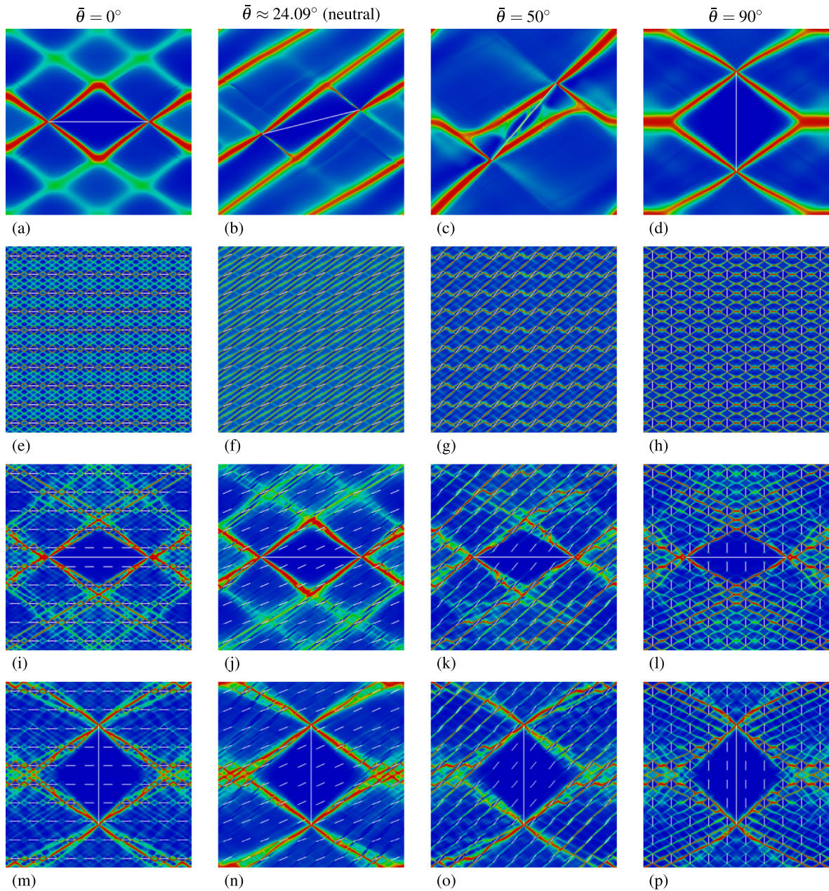
Fig. 19. Maps of damage field \omega revealing shear band patterns in a unit square cell (of side L ) subject to macroscopic straining in the vertical direction and containing different RLIs’ distributions. Upper row: one large (or ‘macro’) RLI ( a = L/4 ); Second row: a periodic distribution of small (or ‘micro’) RLIs ( a = L/40 ); Third row: one large horizontal RLI inside a periodic distribution of small RLIs at different inclinations ( \bar{\theta} = \{0, 24.09, 50, 90\}^\circ ); Lower row: as in the third row, but the large RLI is vertical. The color scale is the same as in Fig. 9.
