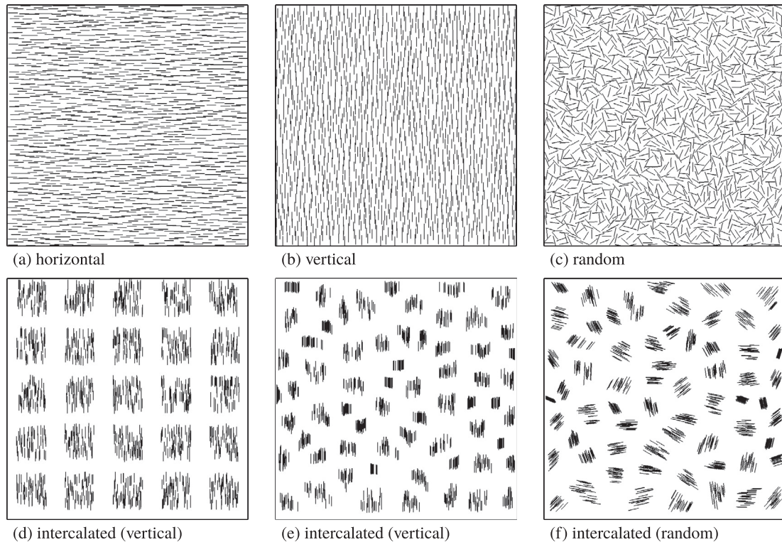
Fig. 7. The roles of RLIs' distribution and volume fraction on the composite mechanical properties are assessed through the estimation of the effective Young's modulus in the vertical direction, E_{\text{eff},y}^{2D} . The figure shows typical RLIs' distributions for the case with 1500 inclusions of length 2a embedded in a square 50a \times 50a unit cell, corresponding to a volume fraction of 4.62%: (a) horizontal, (b) vertical, and (c) random uniformly distributed RLIs; (d, e) vertically intercalated and (f) randomly intercalated RLIs.
