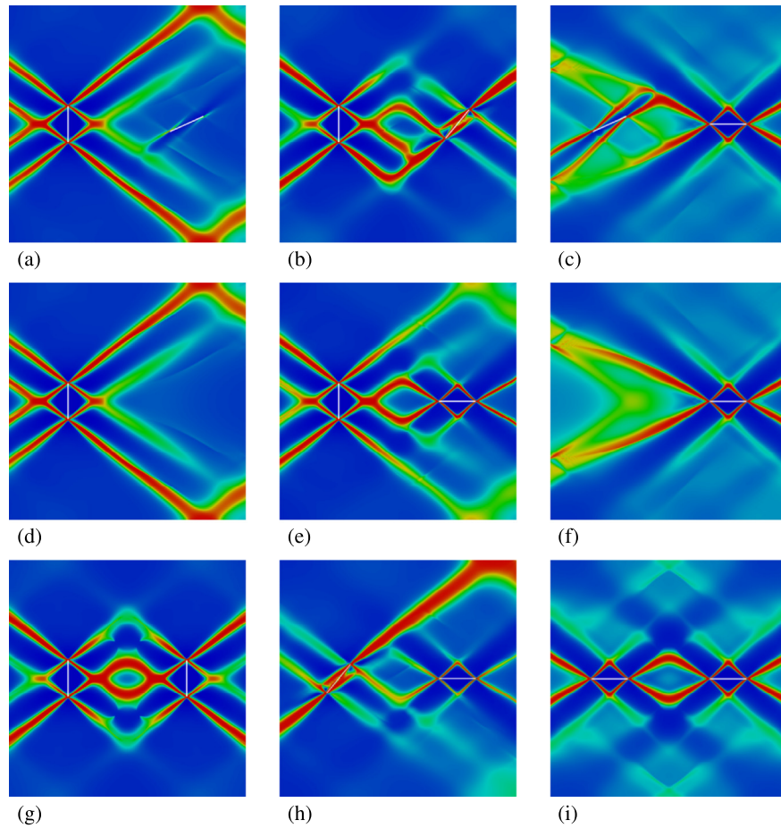
Fig. 11. Localization of damage \omega showing shear bands originating from the interaction of two RLIs at various inclinations: (a) vertical ( \bar{\theta} = 90^\circ ) and at neutral inclination ( \bar{\theta} = \bar{\theta}_n \approx 24.09^\circ ), (b) vertical ( \bar{\theta} = 90^\circ ) and inclined at \bar{\theta} = 50^\circ , (c) neutral ( \bar{\theta} = \bar{\theta}_n \approx 24.09^\circ ) and horizontal ( \bar{\theta} = 0^\circ ), (d) only one vertical inclusion is considered, (e) vertical and horizontal, (f) only one horizontal inclusion is considered, (g) both vertical, (h) inclined at \bar{\theta} = 50^\circ and horizontal, (i) both horizontal. The two cases in panels (d) and (f) with only one inclusion have been included for comparison purposes. The color scale is the same as in Fig. 9.
