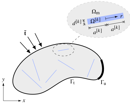
Fig. 1. Two-dimensional schematic of a solid containing rigid line inclusions.
