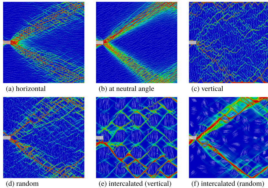
Fig. 17. As for Fig. 16, except that now an imperfection is present on the left edge of the domain as that reported in Fig. 12, where RLIs are not present. RLIs completely change the 'double shear band geometry' visible in Fig. 12 even if the latter still defines, in panels (a) to (d), influence zones for the clusters of shear bands nucleated near the RLIs. The color scale is the same as in Fig. 9.
