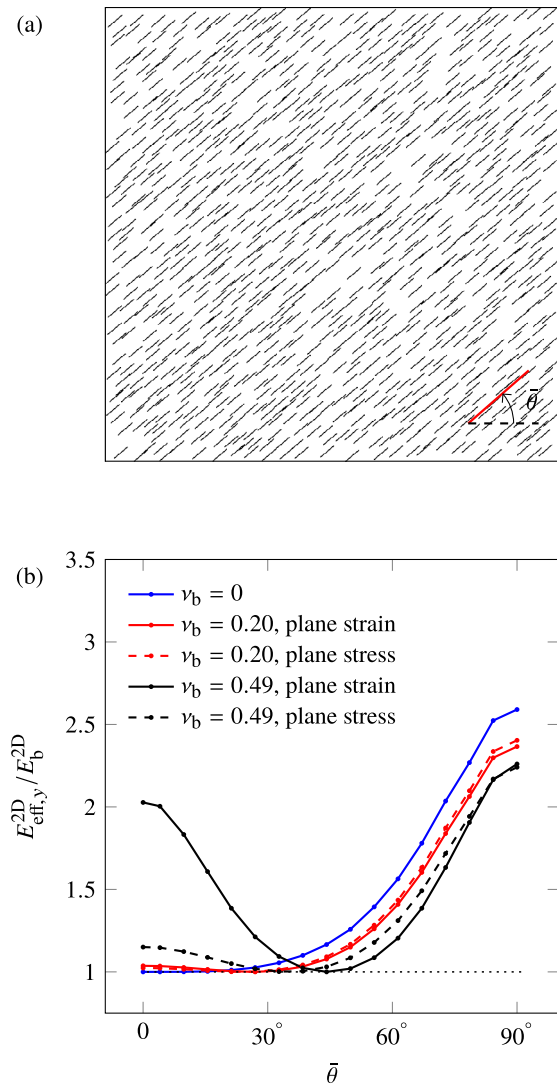
Fig. 6. A square 50a \times 50a unit cell made up of an isotropic elastic matrix material (Young's modulus E_b^{2D} ), containing a random distribution of 1000 equally-inclined rigid line inclusions of length 2a (panel (a)), leads to an equivalent cubic symmetric solid, characterized by an in-plane Young's modulus E_{eff,y}^{2D} , parallel to the (vertical) y -axis. This equivalent stiffness is shown in panel (b) as a function of the inclination \bar{\theta} of the inclusions and for various values of the Poisson's ratio \nu_b of the bulk material. Neutrality of multiple inclusions emerges at the orientation defined by Eq. (33), obtained for a single inclusion embedded in an infinite elastic domain.
