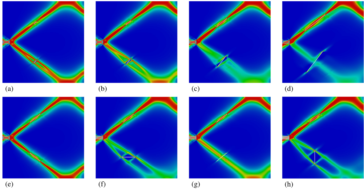
Fig. 15. Maps of damage field \omega revealing interaction of the shear bands nucleated from an imperfection with two RLIs with varying lengths and inclinations. The color scale is the same as in Fig. 9.
