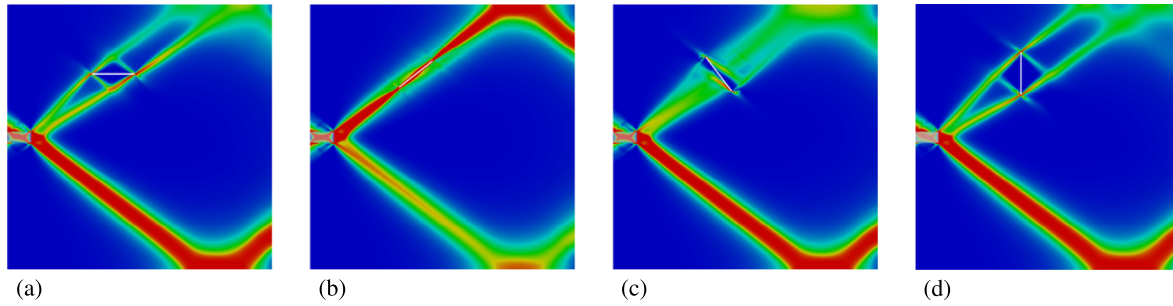
Fig. 13. Maps of damage field \omega revealing interaction of the shear bands nucleated from an imperfection (located at the middle of the left edge of the boundary) with a RLI placed at varying inclinations. The color scale is the same as in Fig. 9.
