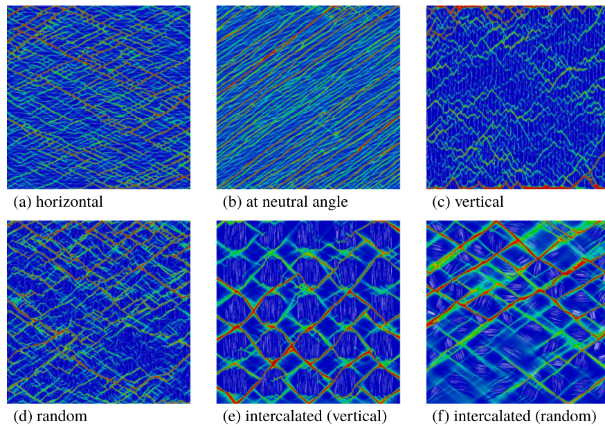
Fig. 16. Maps of damage field \omega revealing shear bands formation from 1500 RLIs at various distributions. RLIs are: (a) horizontal as in Fig. 7(a); (b) inclined at neutral angle \bar{\theta} \approx 24.09^\circ (in a random distribution akin to Fig. 6(a)); (c) vertical as in Fig. 7(b); and (d) randomly inclined as in Fig. 7(c); (e) intercalated vertically as in Fig. 7(d); and (f) intercalated randomly as in Fig. 7(f). The color scale is the same as in Fig. 9.
