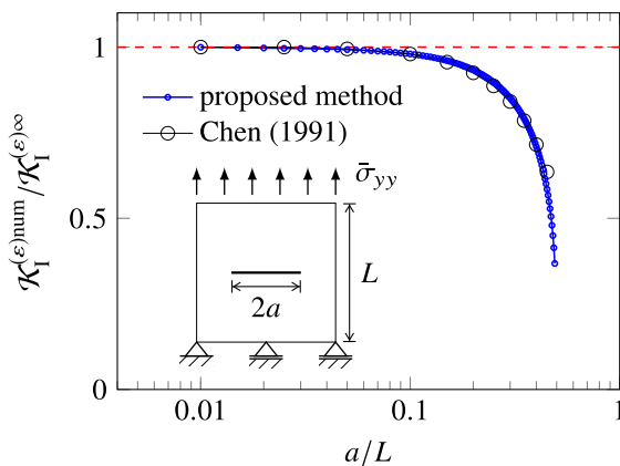
Fig. 4. Effect of the finiteness of the domain size on the stress state at the tip of a RLI. The SIF for a single inclusion in a finite-size domain (Fig. 2(b)) deviates from that related to a single inclusion in an infinite domain (34) (Fig. 2(a)) when the inclusion half-length a is increased relatively to the square domain side L .
