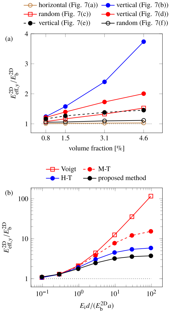
Fig. 8. Predicted effective Young's modulus E_{\text{eff},y}^{2D} of a composite (a) with an increasing number of RLIs for distributions similar to those shown in Fig. 7 and (b) for 1500 vertical inclusions (oriented along the y axis, Fig. 7(b)) as a function of the ratio E_i d / (E_b^{2D} a) . Analytical micromechanical estimates (Voigt, Halpin-Tsai (H-T), and Mori-Tanaka (M-T)) are also included.
