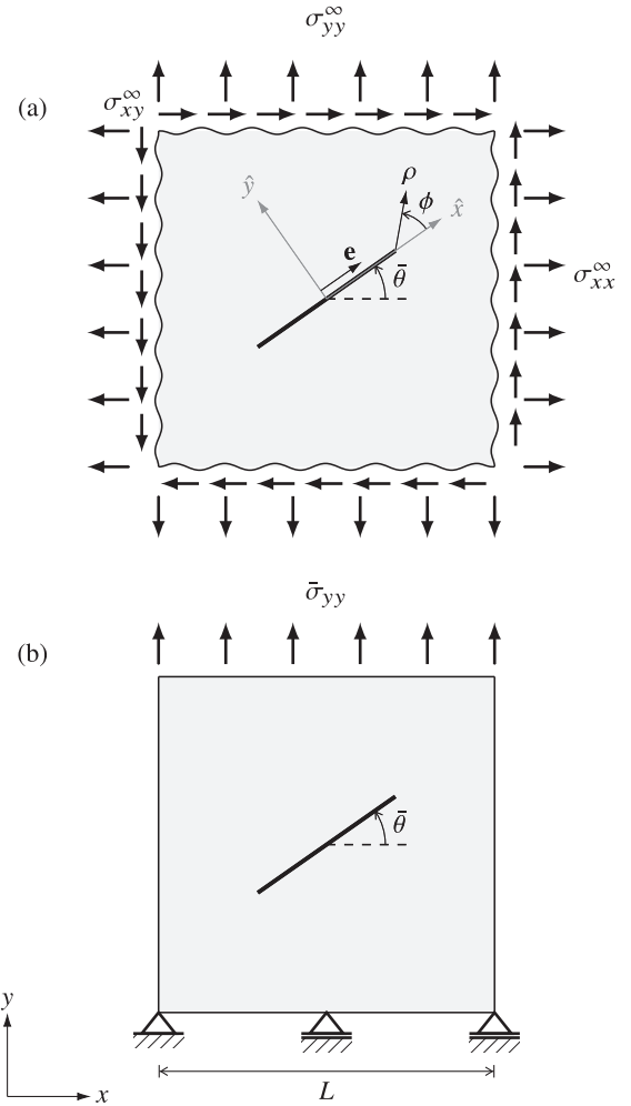
Fig. 2. The two elastic boundary value problems used for the validation of the numerical model: (a) One RLI is embedded in an infinite elastic domain, and (b) the same RLI lies within a square domain of side L . The analytical solution of the elastic boundary value problem in panel (a) is used to validate the numerical model applied to the boundary value problem in panel (b). The unit vector \mathbf{e} = \{\cos\theta, \sin\theta\} is aligned parallel to the inclusion line.
