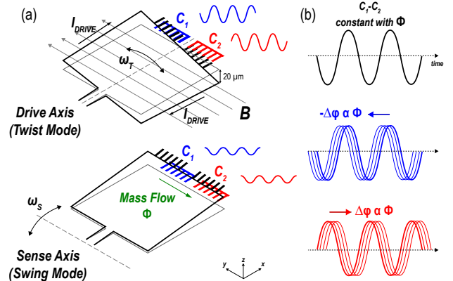
Fig. 1. MEMS Coriolis mass flow sensor (a) operation principle and (b) capacitive signals in the time-domain.
