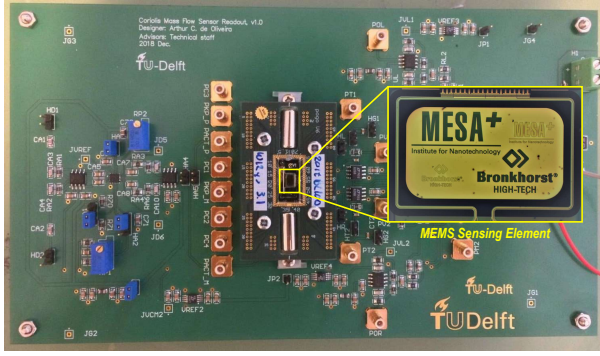
Fig. 3. PCB implementation photo and the MEMS Coriolis mass flow sensor micrograph.
