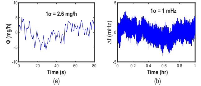
Fig. 5. Stability measurements for (a) mass flow and (b) frequency.
