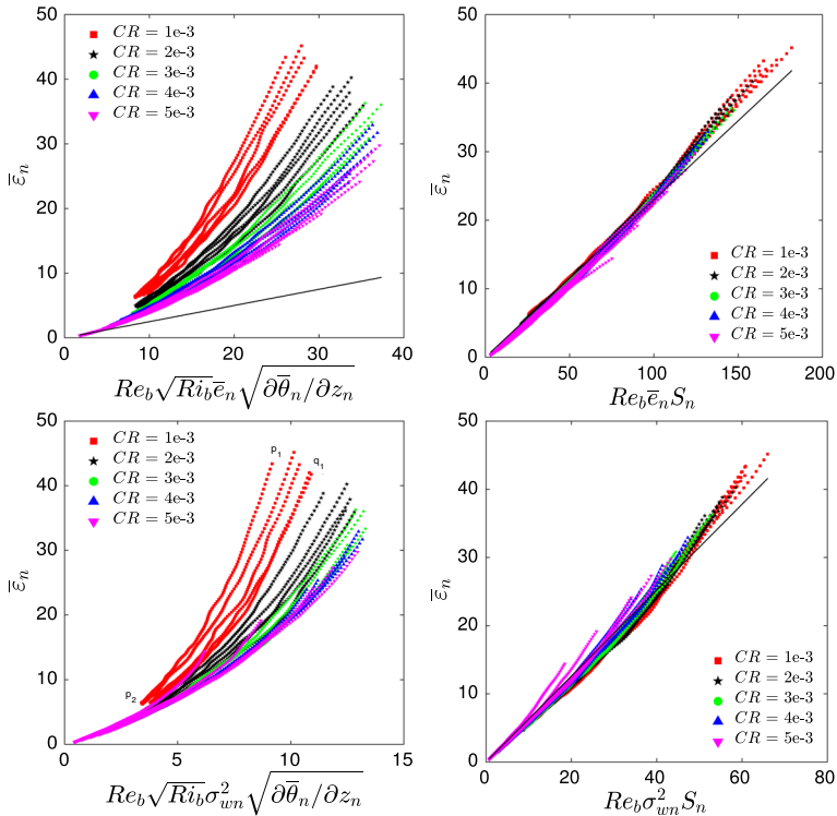
Fig. 4 Variation of normalized energy dissipation rates against normalized \bar{\epsilon}N (top-left panel), normalized \bar{\epsilon}S (top-right panel), normalized \sigma_w^2 N (bottom-left panel), and normalized \sigma_w^2 S (bottom-right panel). Simulated data from five different DNS runs are represented by different coloured symbols in these plots. In the legends, CR represents normalized cooling rates. In the bottom-left panel, the points p_1 and p_2 represent data from z/h = 0.1 and z/h = 0.5 , respectively at non-dimensional time ( T_n ) of 60. Whereas, q_1 is associated with data from z/h = 0.1 at non-dimensional time ( T_n ) of 100
