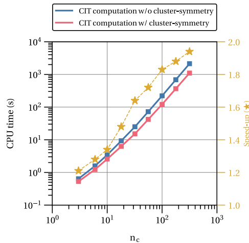
Fig. 27. Comparison between the computational cost of the cluster interaction tensors with and without taking advantage of the cluster-symmetry property. Conditions: 2D problem, n_v = 400 \times 400 , infinitesimal strain formulation with 3 independent strain components.
