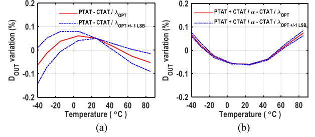
Fig. 17. (a) Measured D_{\text{OUT}} variations over temperature with a 15-A current using a PCB shunt and (b) low-TC metal-alloy shunt.
