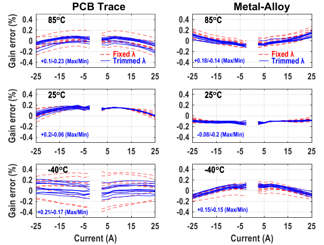
Fig. 18. Measured gain errors at different ambient temperatures for PCB (left) and low-TC metal-alloy shunts (right) w/ and w/o \lambda trimming.
