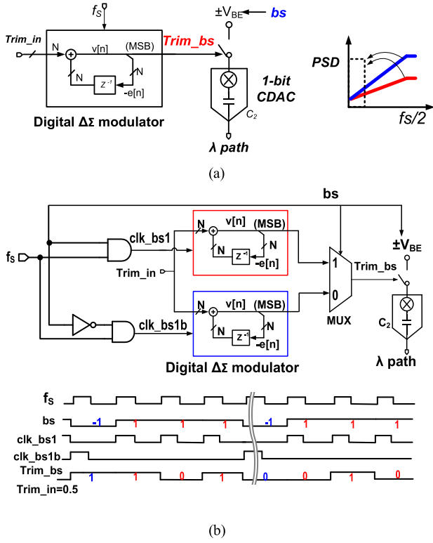
Fig. 10. (a) Simplified diagram of the direct digital \Delta\Sigma trimming. (b) BSC \Delta\Sigma trimming.
