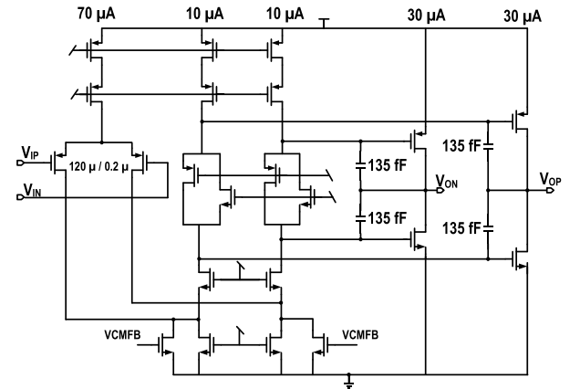
Fig. 9. Circuit implementation of the amplifier in the CCA.
