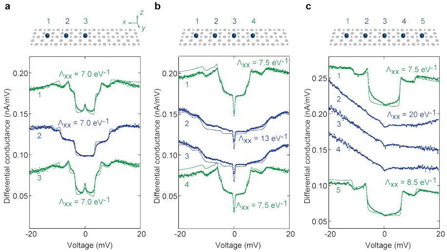
Figure 6.8: Co nanostructures with suppressed and unsuppressed spin excitations. In most cases, Co chains longer than two atoms built on \text{Cu}_2\text{N} showed suppressed spin excitations on the inner atoms (6.1). In a minority of cases (4 out of 20 structures), Co chains up to four atoms long were observed to have unsuppressed spin excitations. This effect was specific to certain locations on the substrate, and is presumably due to variations in local strain induced by subsurface defects. a dI/dV spectra of each atom of a Co trimer and (b) a Co tetramer, as shown in Fig. 6.7c, constructed as an extension of the trimer. Both structures show unsuppressed spin excitations. Simulated spin IETS spectra are shown (solid lines), for all atoms S = 3/2 , \Lambda_{zz} = 6.2 \text{ eV}^{-1} , \Lambda_{yy} = 0 . The trimer may be fitted with \Lambda_{xx} = 7.0 \text{ eV}^{-1} for all atoms: for the tetramer \Lambda_{xx} = 7.5 \text{ eV}^{-1} for the end atoms and 13 \text{ eV}^{-1} for the inner atoms. For both structures the antiferromagnetic spin coupling is 2 \text{ meV} , J_K \rho_s = -0.05 \text{ meV} for inner atoms and -0.15 \text{ meV} for the end atoms. c dI/dV spectra of a Co pentamer constructed as an extension of (b) . In this case no spin IETS steps are seen on the inner atoms: suppression of spin excitations was observed on all structures longer than four atoms. We may conclude that the strain induced by adding a Co atom to the structure overcomes the local lattice strain, pushing all inner atoms of the structure beyond the critical N-Co-N angle that leads to suppression of spin excitations. The end atom spectra may be simulated using a similar model to Fig. 6.3: for all atoms S = 3/2 , J_K \rho_s = -0.05 \text{ meV} , \Lambda_{zz} = 6.2 \text{ eV}^{-1} , \Lambda_{yy} = 0 , the antiferromagnetic spin coupling is 2 \text{ meV} . For the end atoms \Lambda_{xx} = 7.5 and 8.5 \text{ eV}^{-1} , for the inner atoms \Lambda_{xx} = 20 \text{ eV}^{-1} . Note that the anisotropy values are smaller than in Fig. 6.3, illustrating the effect of the local strain.
