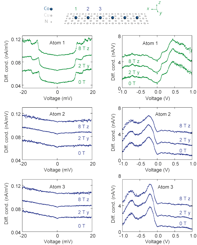
Figure 6.6: Effect of magnetic field on spin and orbital excitation spectra of a Co nanostructure. dI/dV spectra of the same Co hexamer as shown in Fig. 6.4, including data taken with magnetic field applied in the out of plane direction ( z ) and in-plane, perpendicular to the chain direction ( y ). Only the first three atoms are shown. For the end atom spin IETS spectra up to 20 mV, only the expected small Zeeman shift in excitation energies is observed. For the orbital IETS spectra up to 1 V, no change in the spectra is seen with applied field.
