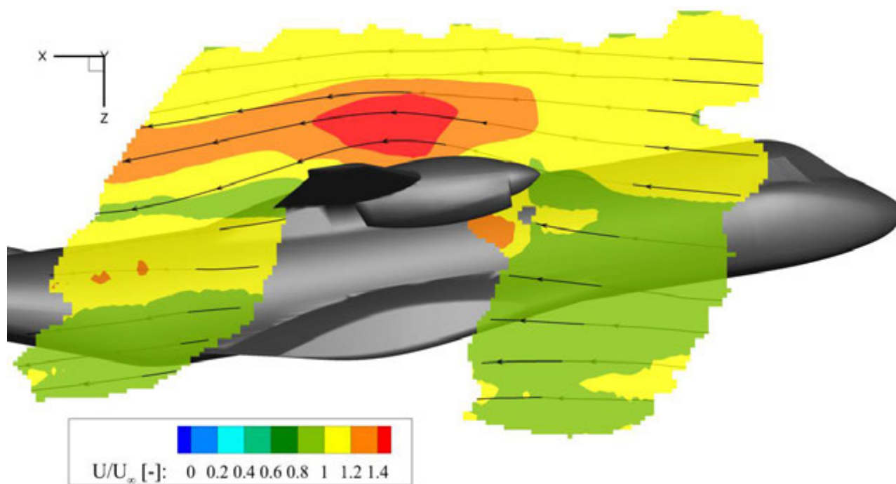
Fig. 5. Streamwise velocity field with streamlines at y/(b/2) = -0.22 .
