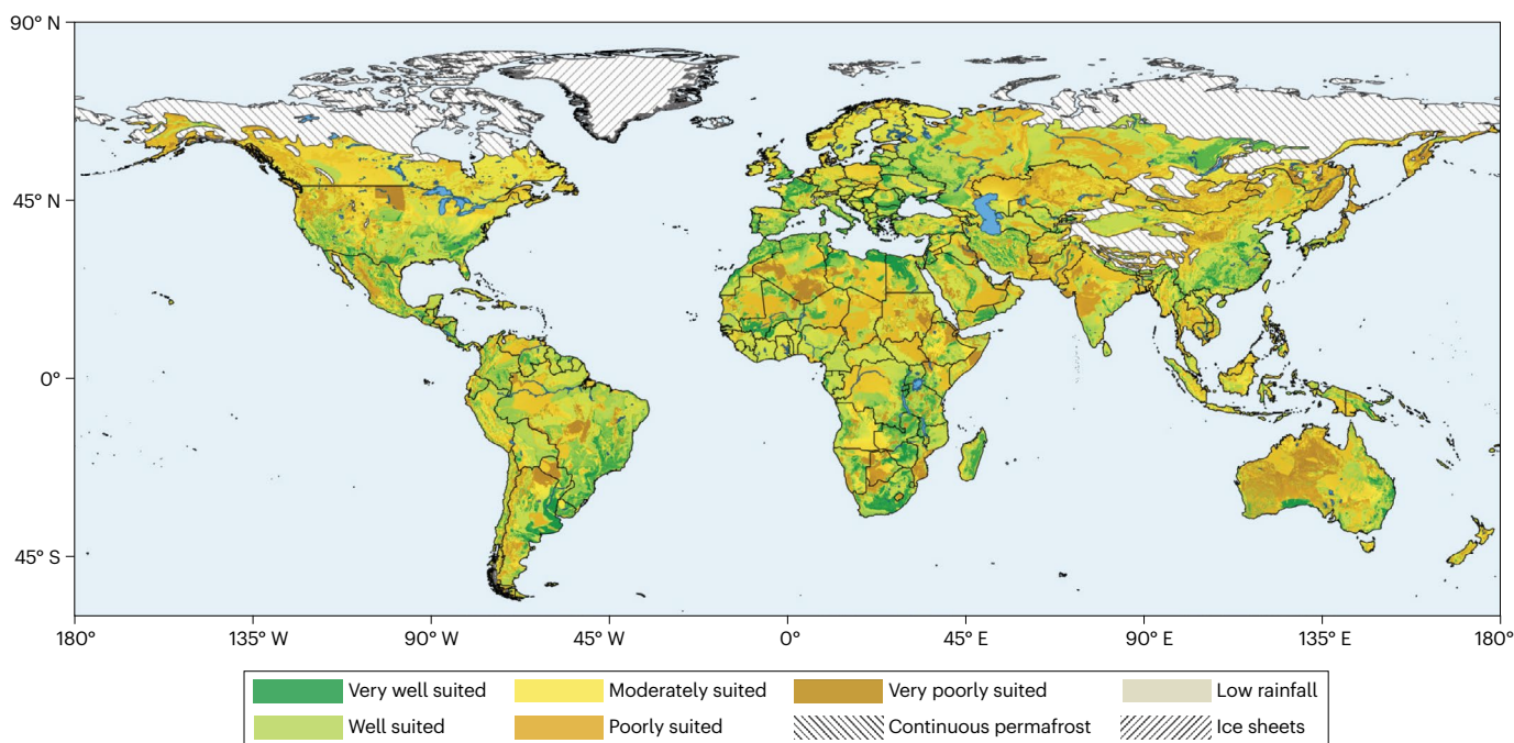
Fig. 2 | Global suitability of shallow geothermal energy. a, Suitability for open-loop shallow geothermal energy (SGE) systems excluding areas with low rainfall 26 and continuous permafrost areas 20 . b, As in part a, but for closed-loop SGE.
