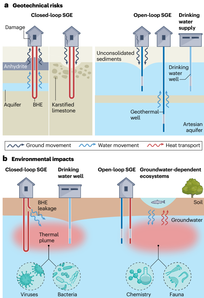
Fig. 5 | Potential geotechnical risks and environmental impacts of shallow geothermal energy systems. a , Potential building damages due to ground uplift caused by anhydrite swelling in the subsurface (left) and sinkholes in areas with karstified limestone (middle), as well as potential impacts on drinking water supply by upwelling of deep groundwater through hydraulic shortcuts (right). b , Potential environmental impacts on groundwater quality and/or groundwater-dependent ecosystems through thermal and/or hydraulic alteration caused by SGE. SGE can pose geotechnical risks, which are reported to be manageable, as well as have only minor impacts on environmental processes as temperature increases are typically in the range of 5–10 K. BHE, borehole heat exchanger; SGE, shallow geothermal energy.
